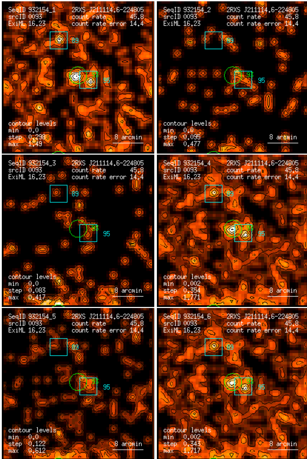
Figure 93: RASS 932154: detection 0093: band rate images, Gaussian filter: (1) PSPC channels 11 – 41, (2) 52 – 90, (3) 91 – 201, (4) 11 – 235, (5) 52 – 201, (6) 11 – 201. Broad band rates in counts/ks. Band rate contour levels in counts/ks/arcmin 2 .
