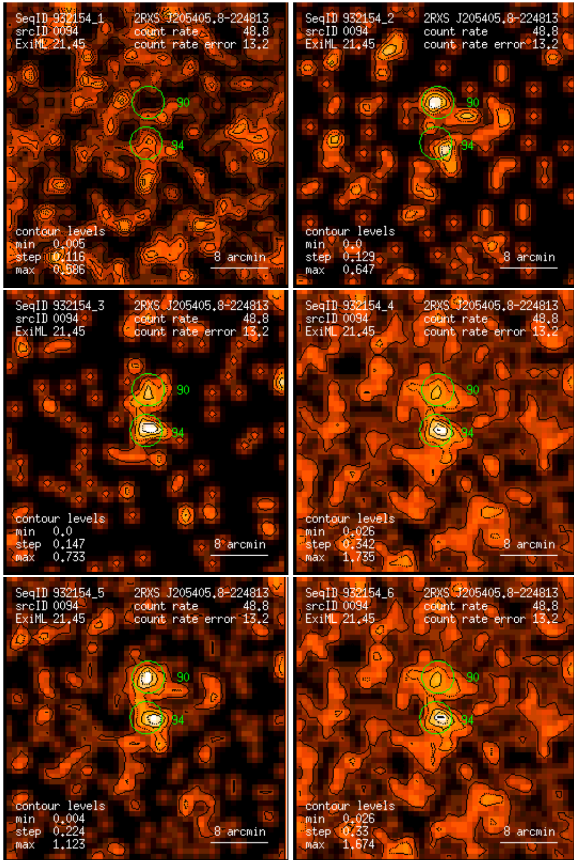
Figure 94: RASS 932154: detection 0094: band rate images, Gaussian filter: (1) PSPC channels 11 – 41, (2) 52 – 90, (3) 91 – 201, (4) 11 – 235, (5) 52 – 201, (6) 11 – 201. Broad band rates in counts/ks. Band rate contour levels in counts/ks/arcmin 2 .
