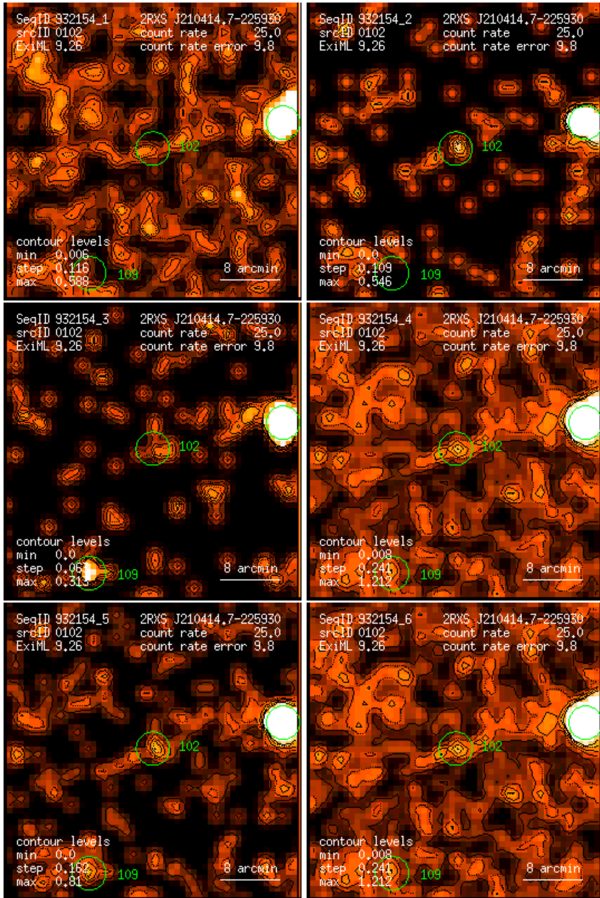
Figure 102: RASS 932154: detection 0102: band rate images, Gaussian filter: (1) PSPC channels 11 – 41, (2) 52 – 90, (3) 91 – 201, (4) 11 – 235, (5) 52 – 201, (6) 11 – 201. Broad band rates in counts/ks. Band rate contour levels in counts/ks/arcmin 2 .
