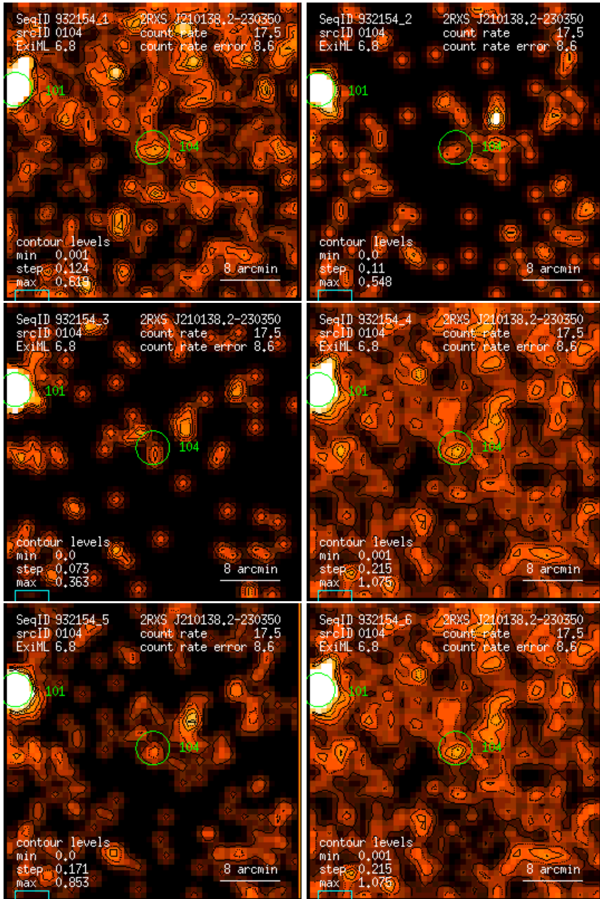
Figure 104: RASS 932154: detection 0104: band rate images, Gaussian filter: (1) PSPC channels 11 – 41, (2) 52 – 90, (3) 91 – 201, (4) 11 – 235, (5) 52 – 201, (6) 11 – 201. Broad band rates in counts/ks. Band rate contour levels in counts/ks/arcmin 2 .
