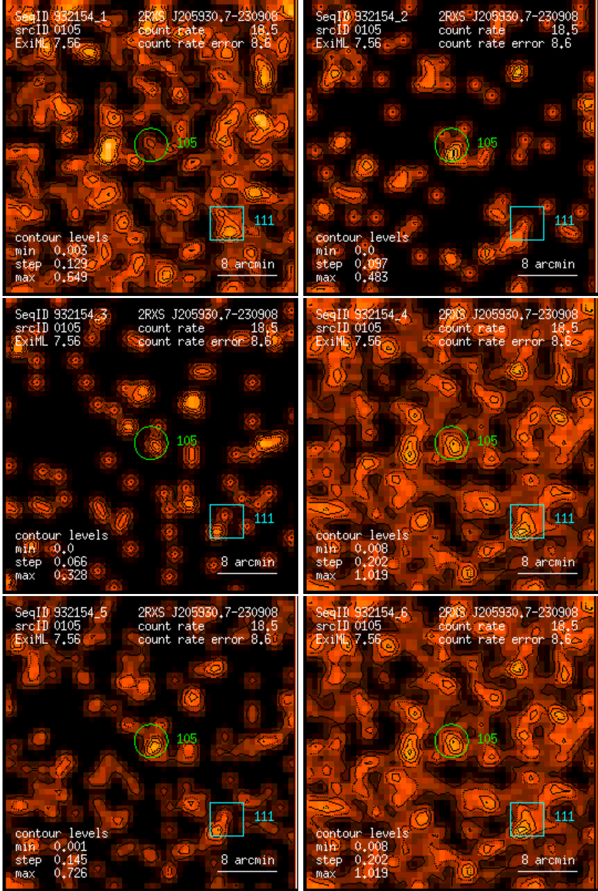
Figure 105: RASS 932154: detection 0105: band rate images, Gaussian filter: (1) PSPC channels 11 – 41, (2) 52 – 90, (3) 91 – 201, (4) 11 – 235, (5) 52 – 201, (6) 11 – 201. Broad band rates in counts/ks. Band rate contour levels in counts/ks/arcmin 2 .
