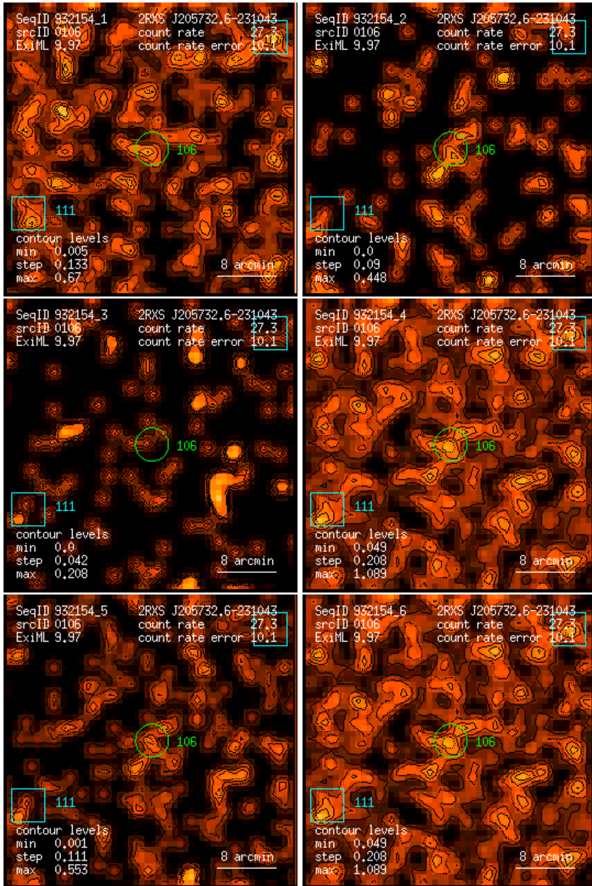
Figure 106: RASS 932154: detection 0106: band rate images, Gaussian filter: (1) PSPC channels 11 – 41, (2) 52 – 90, (3) 91 – 201, (4) 11 – 235, (5) 52 – 201, (6) 11 – 201. Broad band rates in counts/ks. Band rate contour levels in counts/ks/arcmin 2 .
