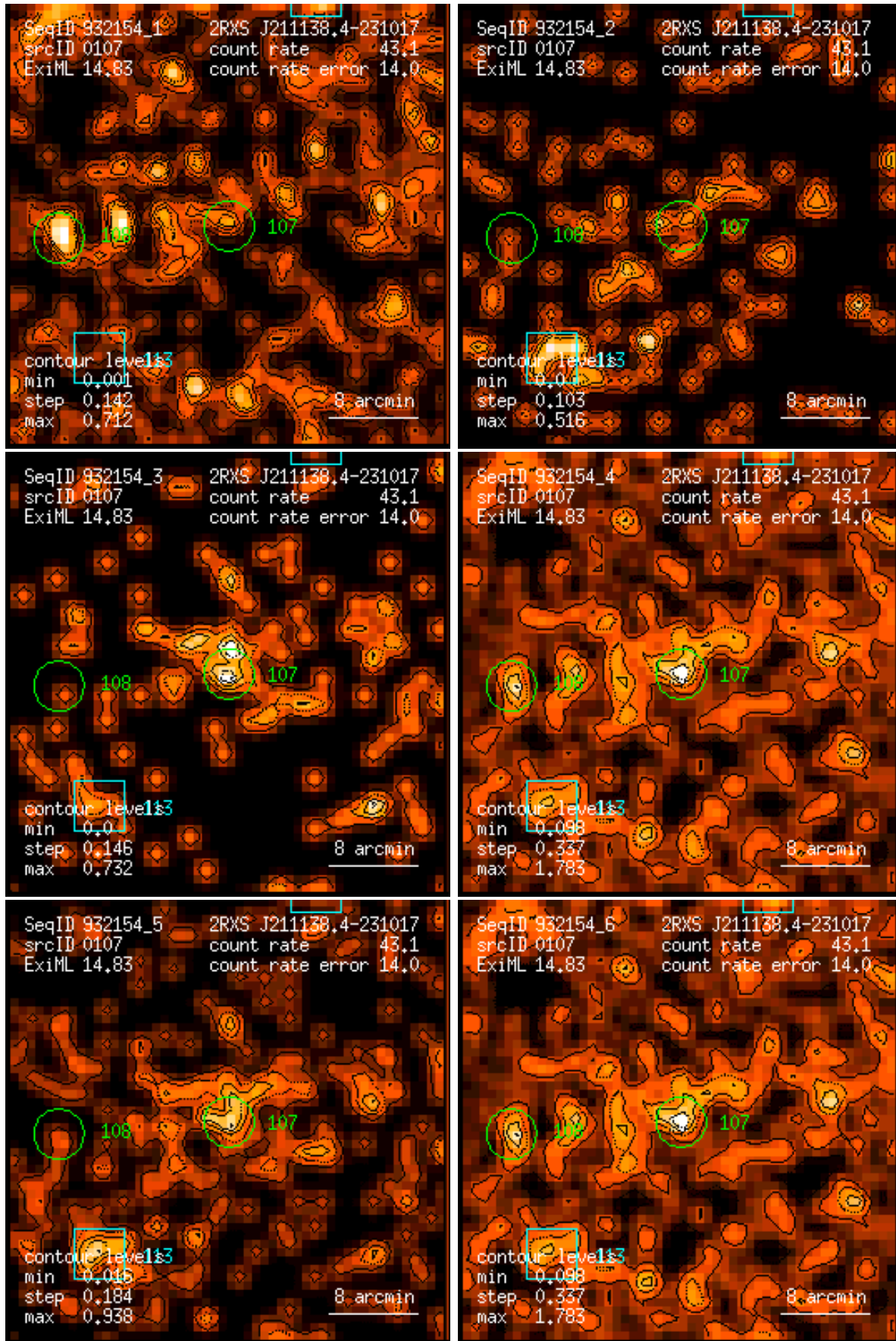
Figure 107: RASS 932154: detection 0107: band rate images, Gaussian filter: (1) PSPC channels 11 – 41, (2) 52 – 90, (3) 91 – 201, (4) 11 – 235, (5) 52 – 201, (6) 11 – 201. Broad band rates in counts/ks. Band rate contour levels in counts/ks/arcmin 2 .
