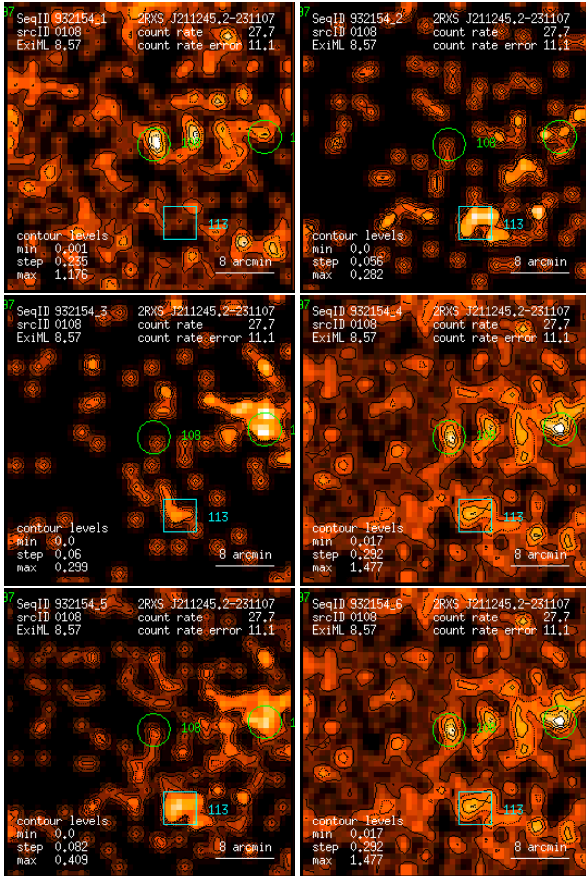
Figure 108: RASS 932154: detection 0108: band rate images, Gaussian filter: (1) PSPC channels 11 – 41, (2) 52 – 90, (3) 91 – 201, (4) 11 – 235, (5) 52 – 201, (6) 11 – 201. Broad band rates in counts/ks. Band rate contour levels in counts/ks/arcmin 2 .
