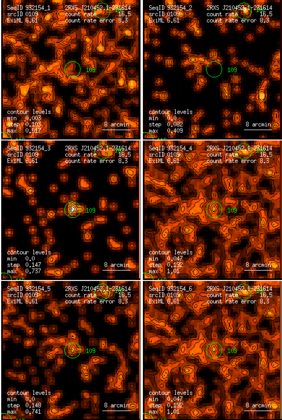
Figure 109: RASS 932154: detection 0109: band rate images, Gaussian filter: (1) PSPC channels 11 – 41, (2) 52 – 90, (3) 91 – 201, (4) 11 – 235, (5) 52 – 201, (6) 11 – 201. Broad band rates in counts/ks. Band rate contour levels in counts/ks/arcmin 2 .
