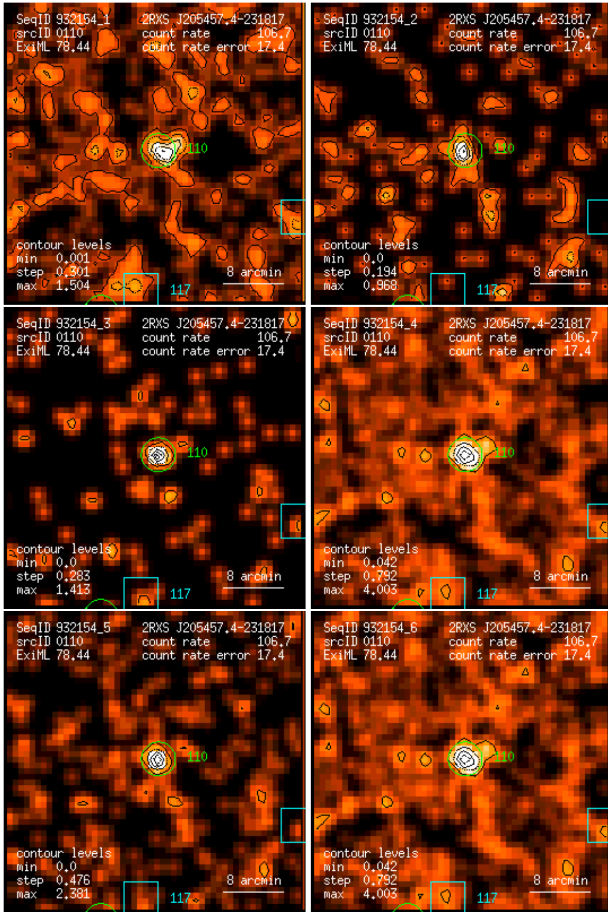
Figure 110: RASS 932154: detection 0110: band rate images, Gaussian filter: (1) PSPC channels 11 – 41, (2) 52 – 90, (3) 91 – 201, (4) 11 – 235, (5) 52 – 201, (6) 11 – 201. Broad band rates in counts/ks. Band rate contour levels in counts/ks/arcmin 2 .
