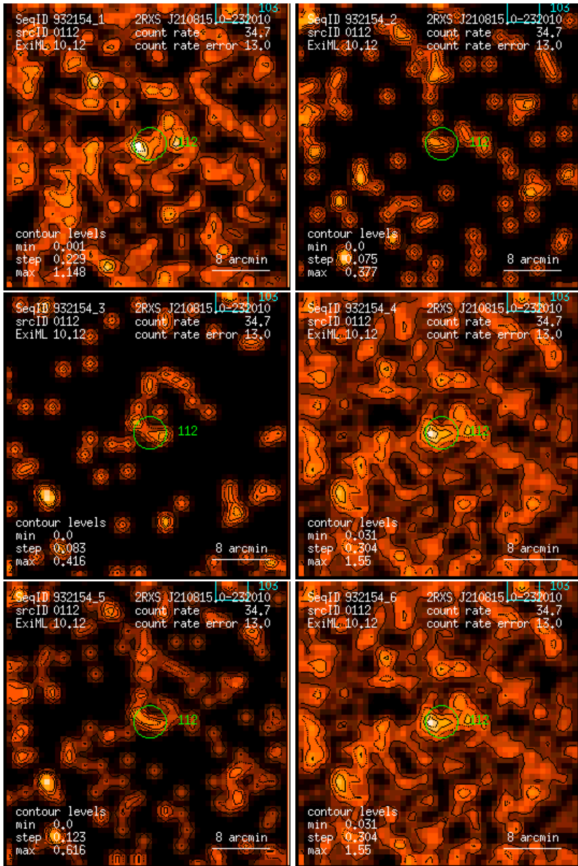
Figure 112: RASS 932154: detection 0112: band rate images, Gaussian filter: (1) PSPC channels 11 – 41, (2) 52 – 90, (3) 91 – 201, (4) 11 – 235, (5) 52 – 201, (6) 11 – 201. Broad band rates in counts/ks. Band rate contour levels in counts/ks/arcmin 2 .
