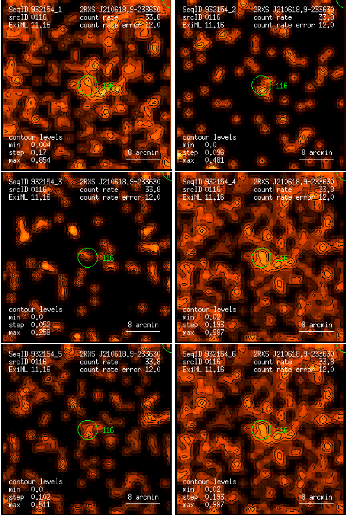
Figure 116: RASS 932154: detection 0116: band rate images, Gaussian filter: (1) PSPC channels 11 – 41, (2) 52 – 90, (3) 91 – 201, (4) 11 – 235, (5) 52 – 201, (6) 11 – 201. Broad band rates in counts/ks. Band rate contour levels in counts/ks/arcmin 2 .
