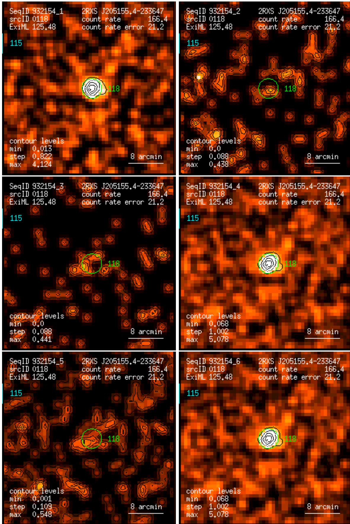
Figure 118: RASS 932154: detection 0118: band rate images, Gaussian filter: (1) PSPC channels 11 – 41, (2) 52 – 90, (3) 91 – 201, (4) 11 – 235, (5) 52 – 201, (6) 11 – 201. Broad band rates in counts/ks. Band rate contour levels in counts/ks/arcmin 2 .
