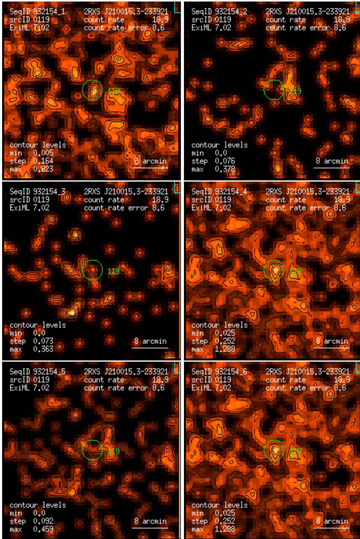
Figure 119: RASS 932154: detection 0119: band rate images, Gaussian filter: (1) PSPC channels 11 – 41, (2) 52 – 90, (3) 91 – 201, (4) 11 – 235, (5) 52 – 201, (6) 11 – 201. Broad band rates in counts/ks. Band rate contour levels in counts/ks/arcmin 2 .
