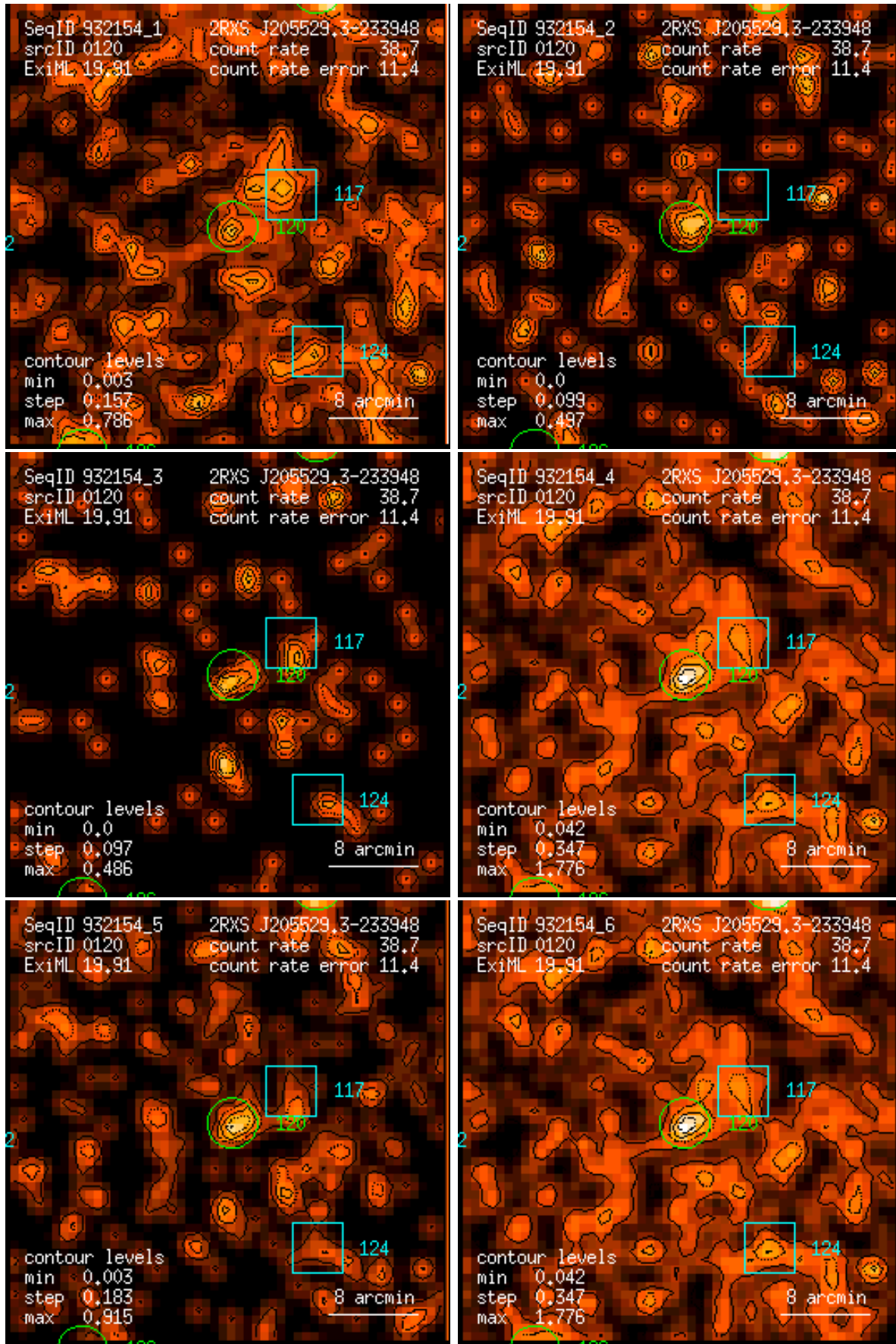
Figure 120: RASS 932154: detection 0120: band rate images, Gaussian filter: (1) PSPC channels 11 – 41, (2) 52 – 90, (3) 91 – 201, (4) 11 – 235, (5) 52 – 201, (6) 11 – 201. Broad band rates in counts/ks. Band rate contour levels in counts/ks/arcmin 2 .
