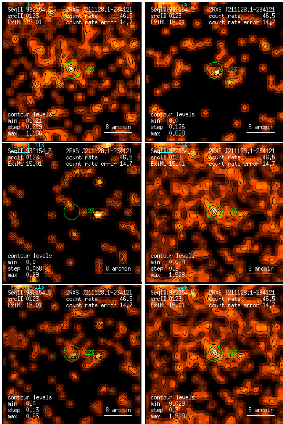
Figure 123: RASS 932154: detection 0123: band rate images, Gaussian filter: (1) PSPC channels 11 – 41, (2) 52 – 90, (3) 91 – 201, (4) 11 – 235, (5) 52 – 201, (6) 11 – 201. Broad band rates in counts/ks. Band rate contour levels in counts/ks/arcmin 2 .
