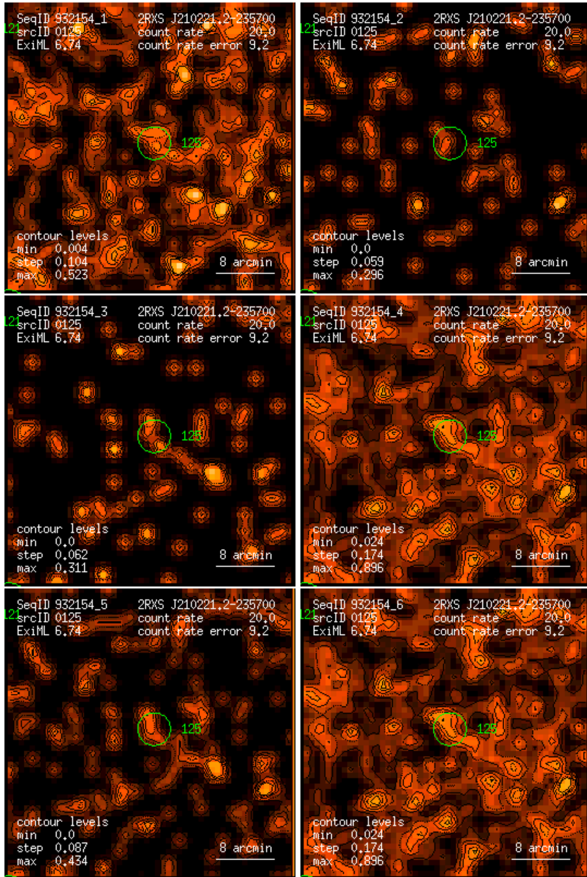
Figure 125: RASS 932154: detection 0125: band rate images, Gaussian filter: (1) PSPC channels 11 – 41, (2) 52 – 90, (3) 91 – 201, (4) 11 – 235, (5) 52 – 201, (6) 11 – 201. Broad band rates in counts/ks. Band rate contour levels in counts/ks/arcmin 2 .
