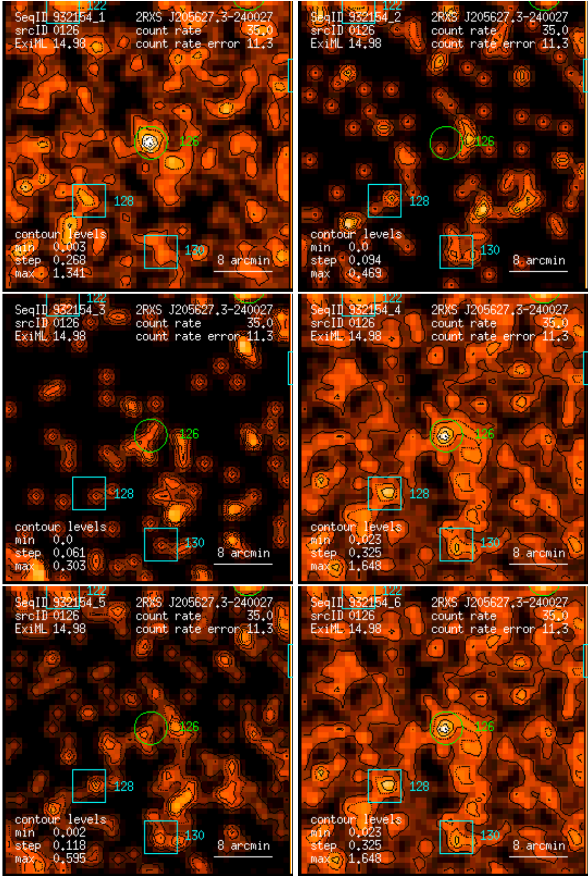
Figure 126: RASS 932154: detection 0126: band rate images, Gaussian filter: (1) PSPC channels 11 – 41, (2) 52 – 90, (3) 91 – 201, (4) 11 – 235, (5) 52 – 201, (6) 11 – 201. Broad band rates in counts/ks. Band rate contour levels in counts/ks/arcmin 2 .
