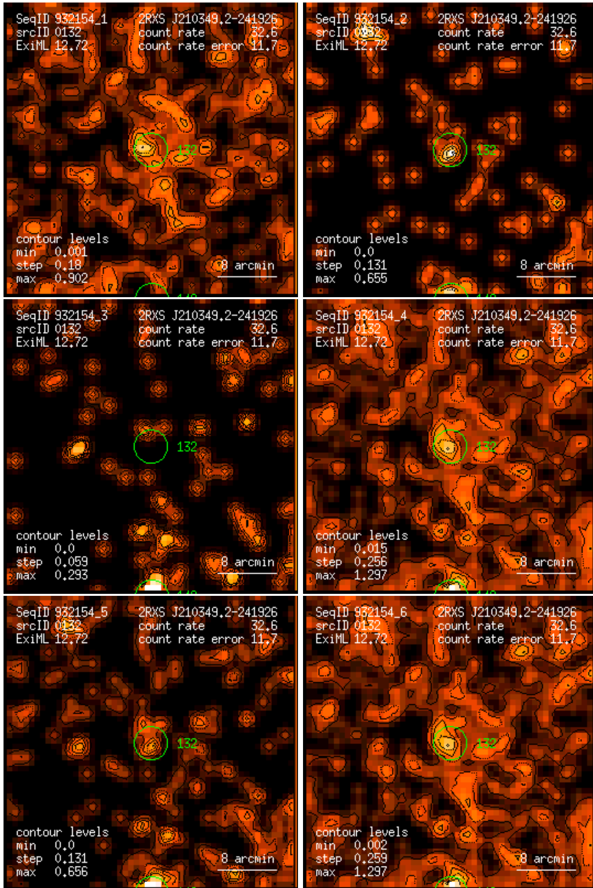
Figure 132: RASS 932154: detection 0132: band rate images, Gaussian filter: (1) PSPC channels 11 – 41, (2) 52 – 90, (3) 91 – 201, (4) 11 – 235, (5) 52 – 201, (6) 11 – 201. Broad band rates in counts/ks. Band rate contour levels in counts/ks/arcmin 2 .
