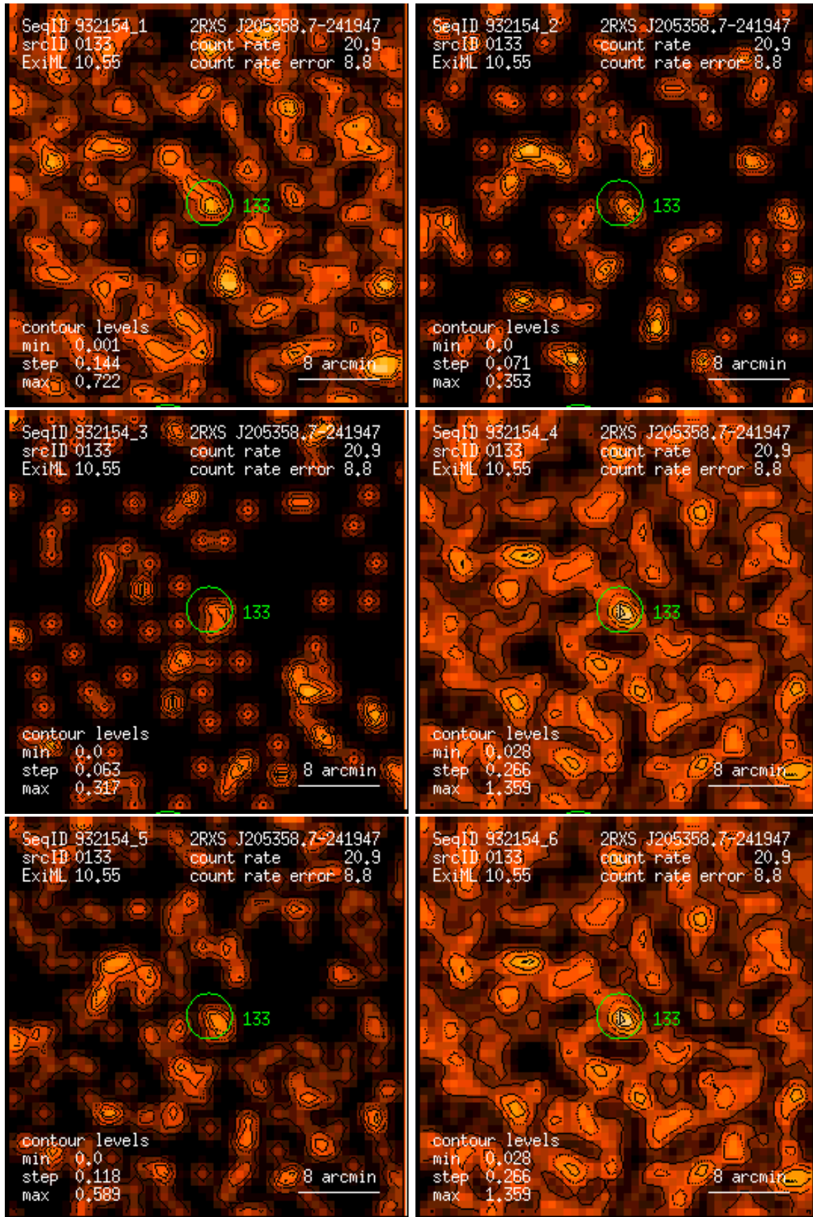
Figure 133: RASS 932154: detection 0133: band rate images, Gaussian filter: (1) PSPC channels 11 – 41, (2) 52 – 90, (3) 91 – 201, (4) 11 – 235, (5) 52 – 201, (6) 11 – 201. Broad band rates in counts/ks. Band rate contour levels in counts/ks/arcmin 2 .
