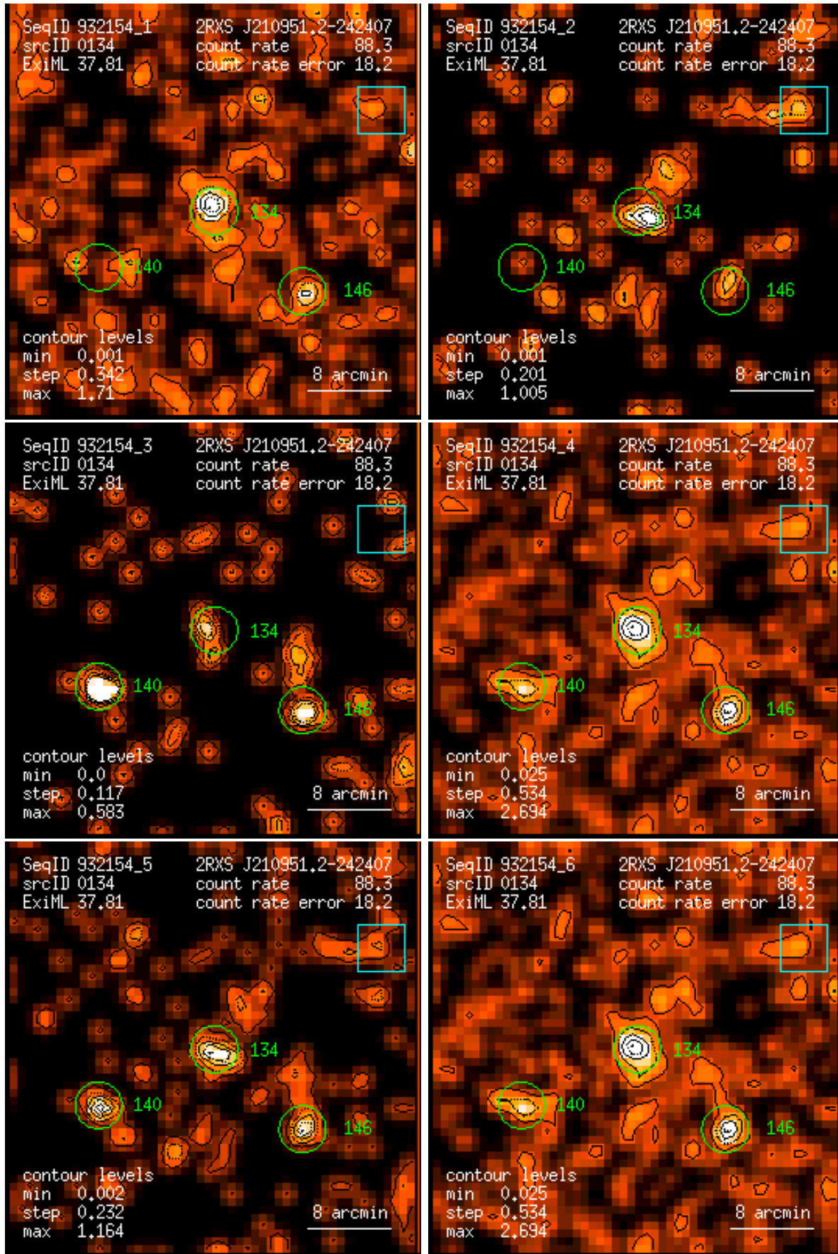
Figure 134: RASS 932154: detection 0134: band rate images, Gaussian filter: (1) PSPC channels 11 – 41, (2) 52 – 90, (3) 91 – 201, (4) 11 – 235, (5) 52 – 201, (6) 11 – 201. Broad band rates in counts/ks. Band rate contour levels in counts/ks/arcmin 2 .
