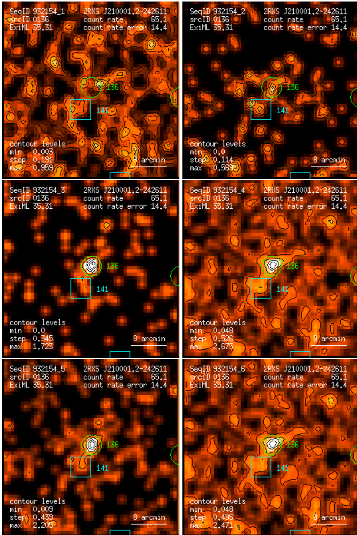
Figure 136: RASS 932154: detection 0136: band rate images, Gaussian filter: (1) PSPC channels 11 – 41, (2) 52 – 90, (3) 91 – 201, (4) 11 – 235, (5) 52 – 201, (6) 11 – 201. Broad band rates in counts/ks. Band rate contour levels in counts/ks/arcmin 2 .
