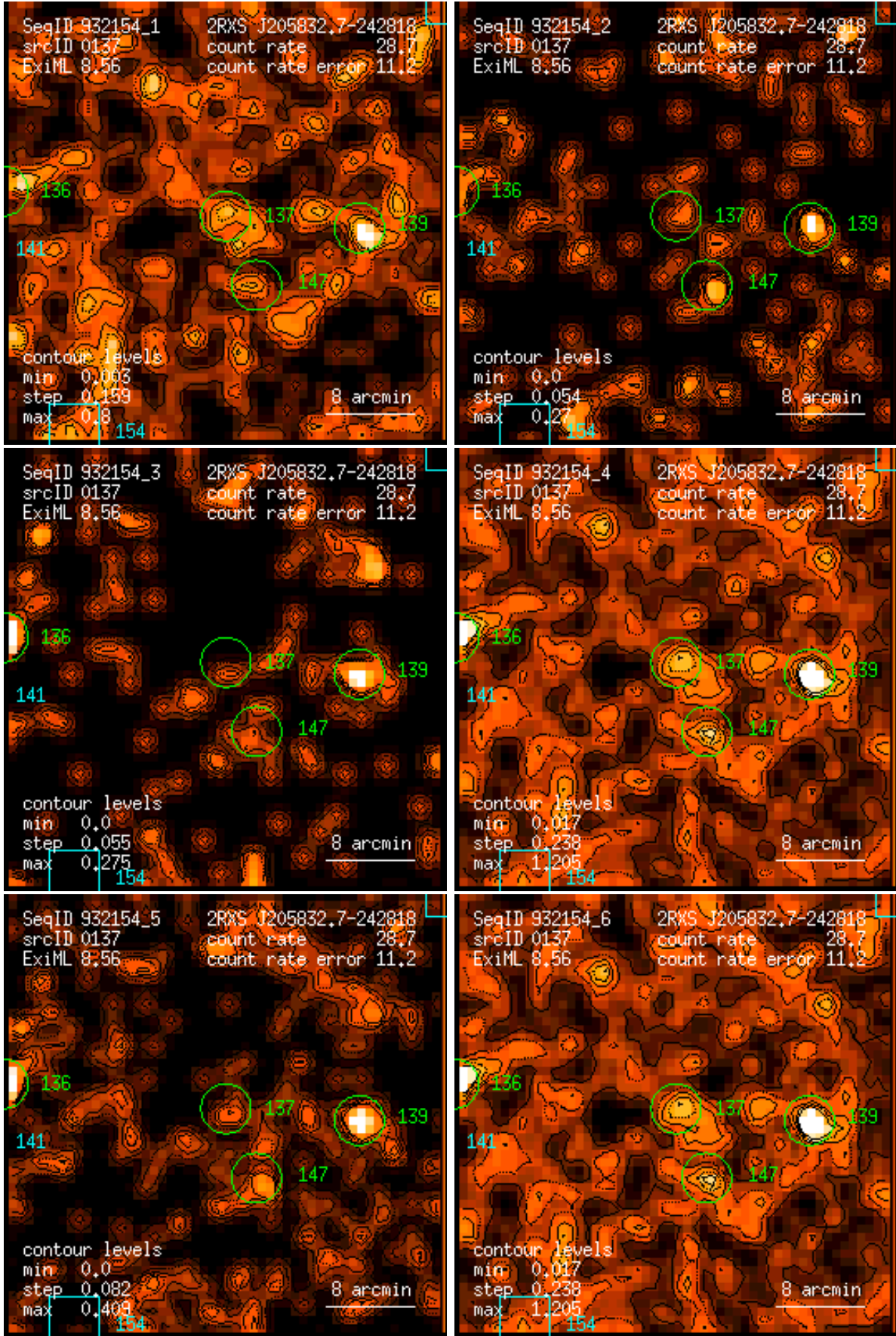
Figure 137: RASS 932154: detection 0137: band rate images, Gaussian filter: (1) PSPC channels 11 – 41, (2) 52 – 90, (3) 91 – 201, (4) 11 – 235, (5) 52 – 201, (6) 11 – 201. Broad band rates in counts/ks. Band rate contour levels in counts/ks/arcmin 2 .
