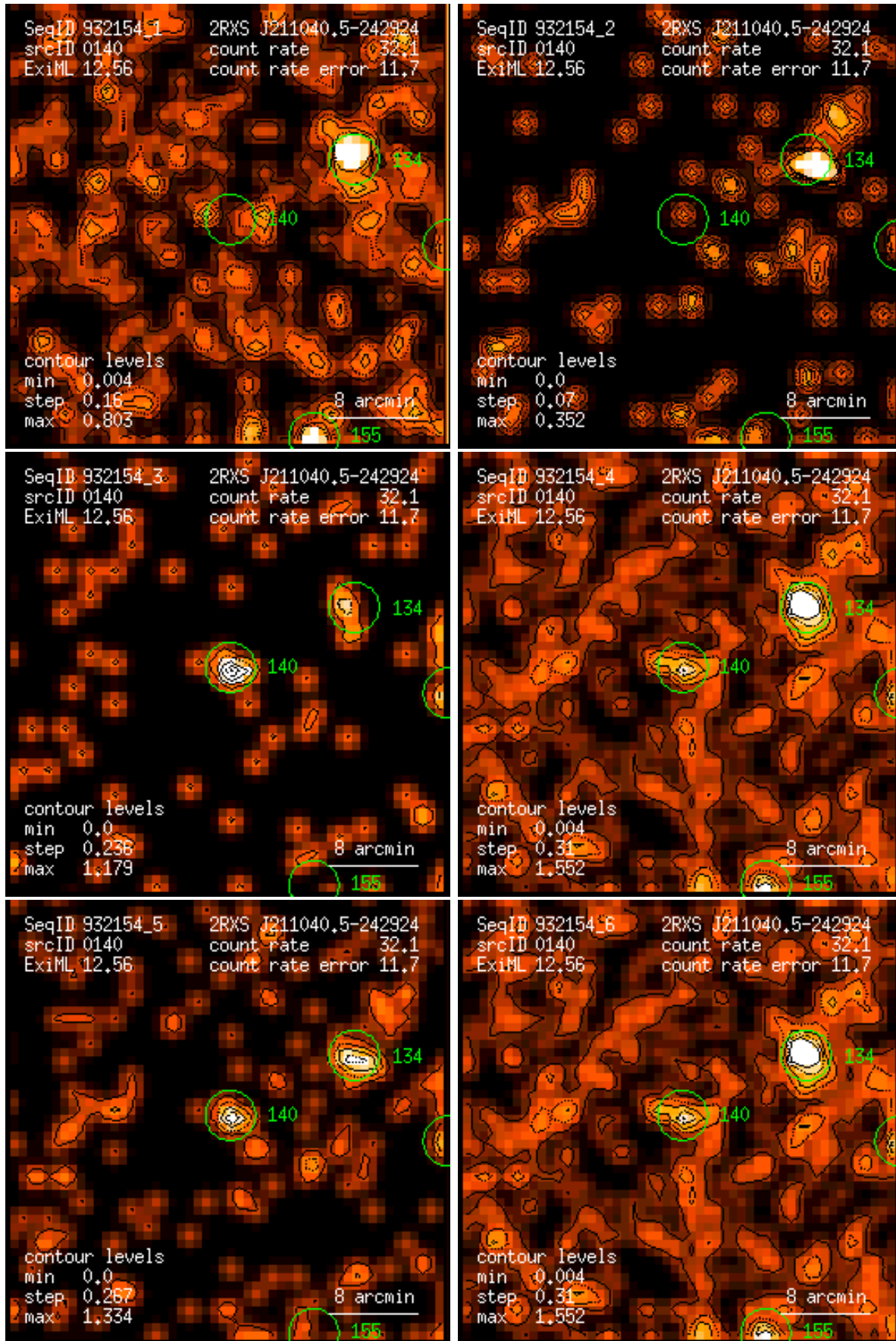
Figure 140: RASS 932154: detection 0140: band rate images, Gaussian filter: (1) PSPC channels 11 – 41, (2) 52 – 90, (3) 91 – 201, (4) 11 – 235, (5) 52 – 201, (6) 11 – 201. Broad band rates in counts/ks. Band rate contour levels in counts/ks/arcmin 2 .
