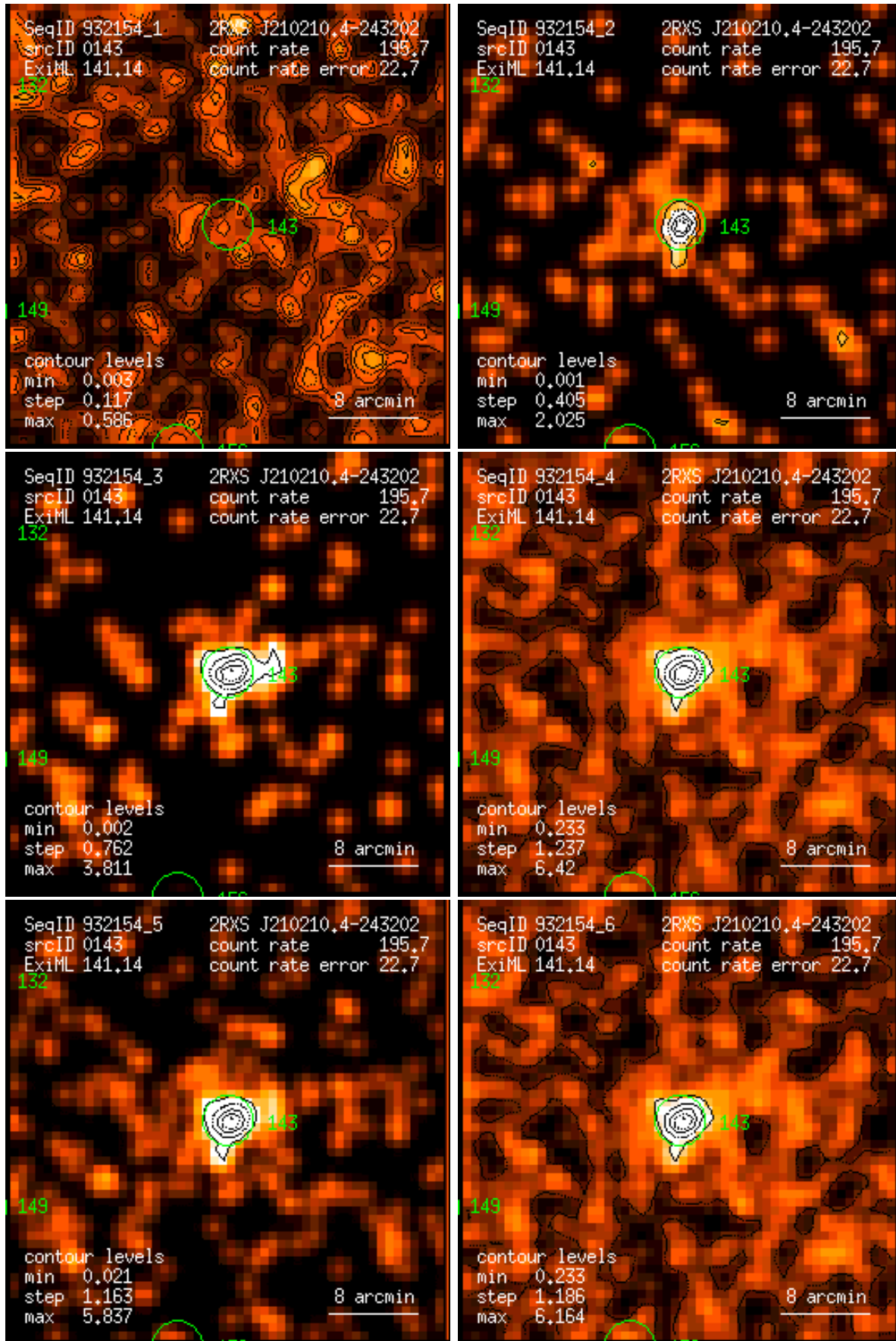
Figure 143: RASS 932154: detection 0143: band rate images, Gaussian filter: (1) PSPC channels 11 – 41, (2) 52 – 90, (3) 91 – 201, (4) 11 – 235, (5) 52 – 201, (6) 11 – 201. Broad band rates in counts/ks. Band rate contour levels in counts/ks/arcmin 2 .
