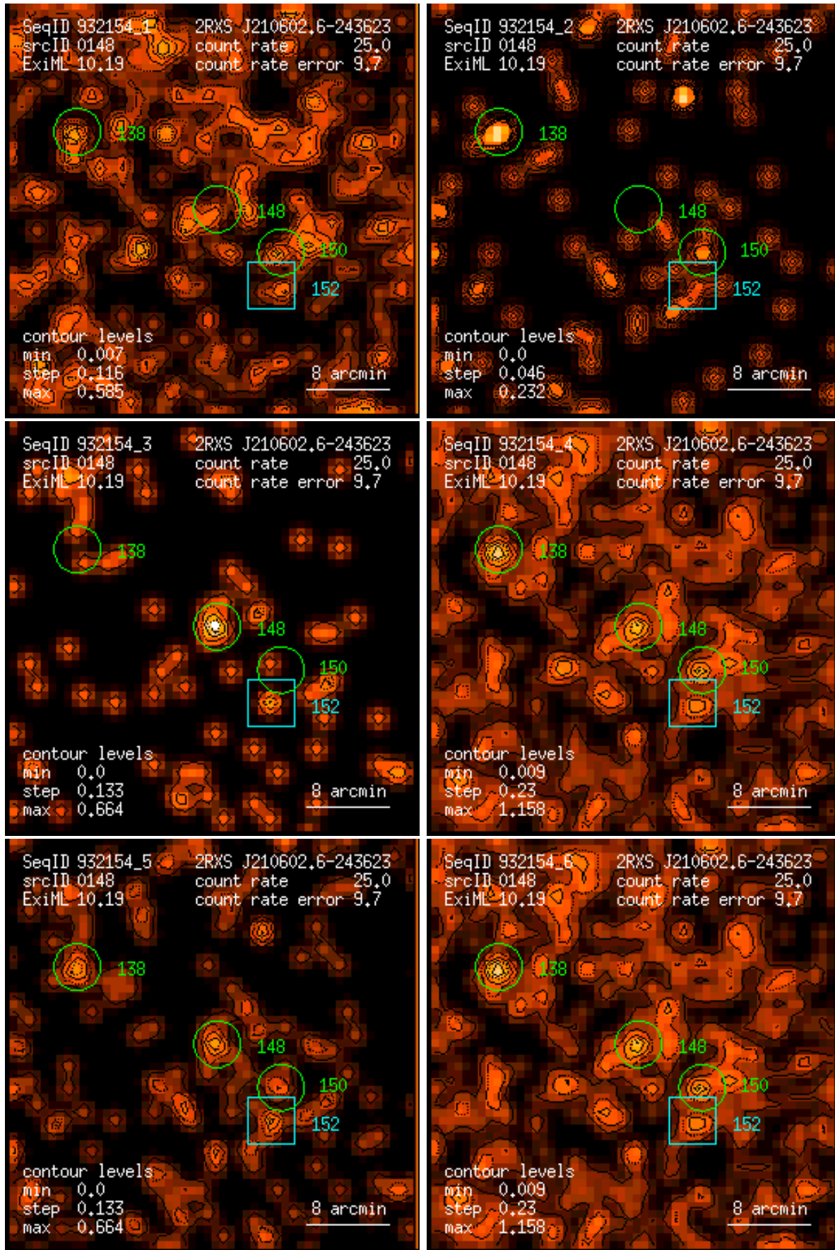
Figure 148: RASS 932154: detection 0148: band rate images, Gaussian filter: (1) PSPC channels 11 – 41, (2) 52 – 90, (3) 91 – 201, (4) 11 – 235, (5) 52 – 201, (6) 11 – 201. Broad band rates in counts/ks. Band rate contour levels in counts/ks/arcmin 2 .
