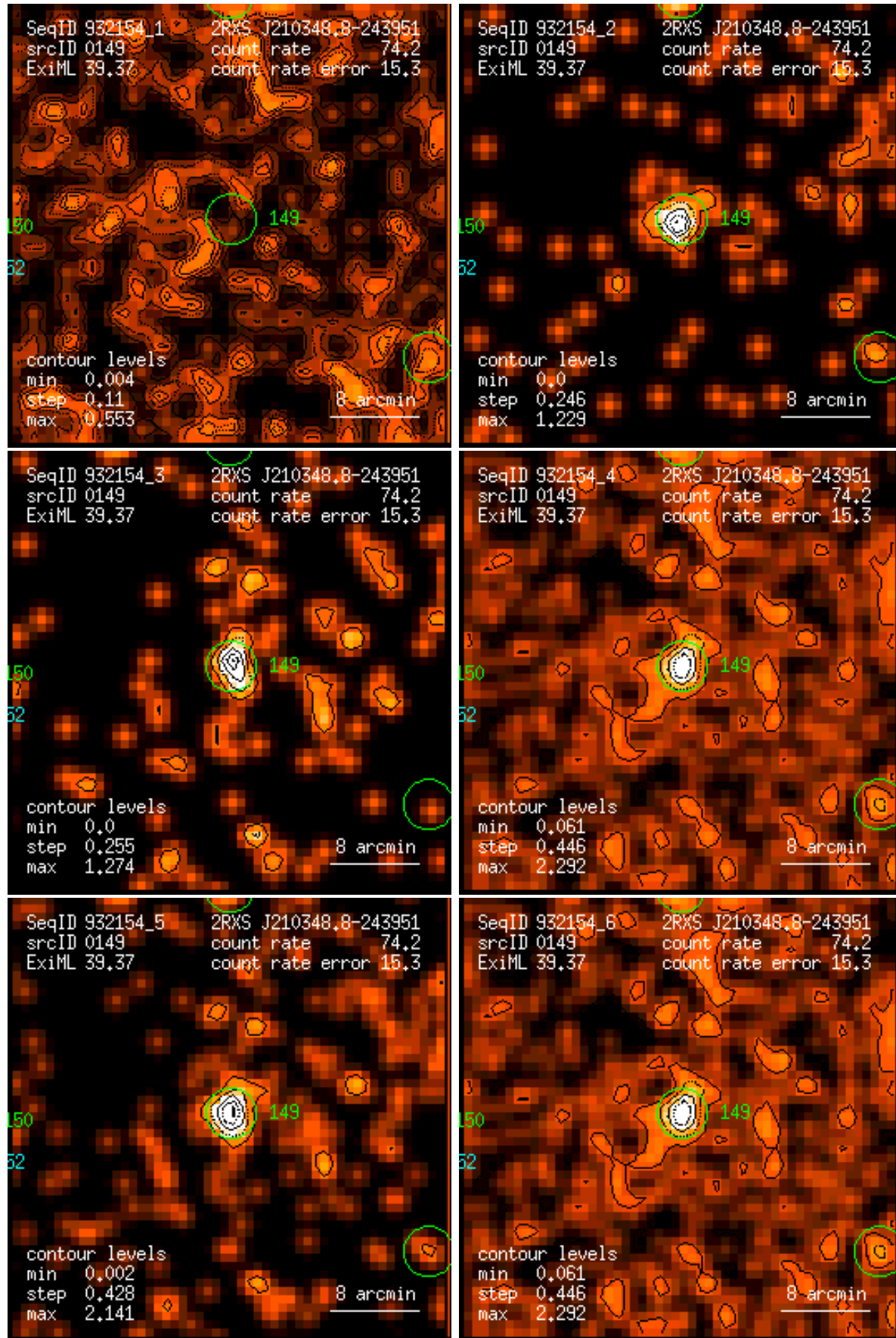
Figure 149: RASS 932154: detection 0149: band rate images, Gaussian filter: (1) PSPC channels 11 – 41, (2) 52 – 90, (3) 91 – 201, (4) 11 – 235, (5) 52 – 201, (6) 11 – 201. Broad band rates in counts/ks. Band rate contour levels in counts/ks/arcmin 2 .
