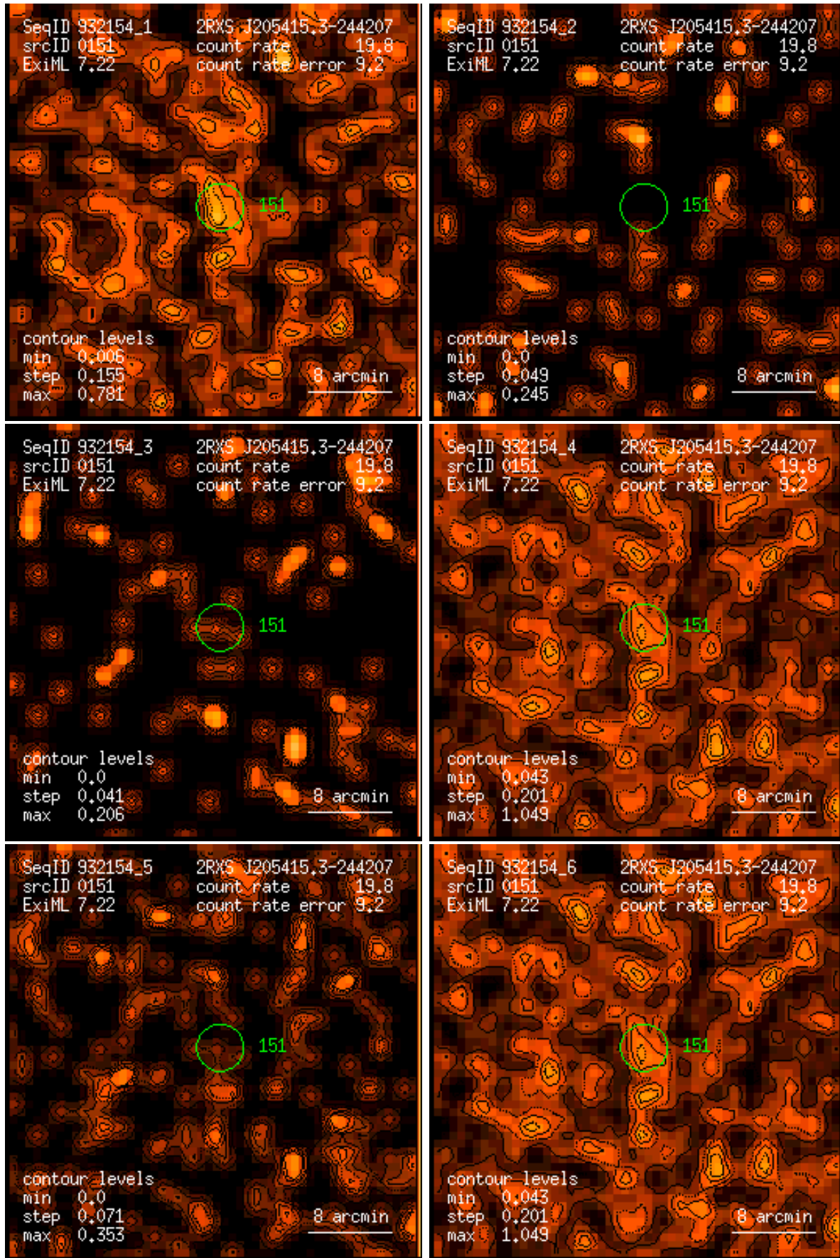
Figure 151: RASS 932154: detection 0151: band rate images, Gaussian filter: (1) PSPC channels 11 – 41, (2) 52 – 90, (3) 91 – 201, (4) 11 – 235, (5) 52 – 201, (6) 11 – 201. Broad band rates in counts/ks. Band rate contour levels in counts/ks/arcmin 2 .
