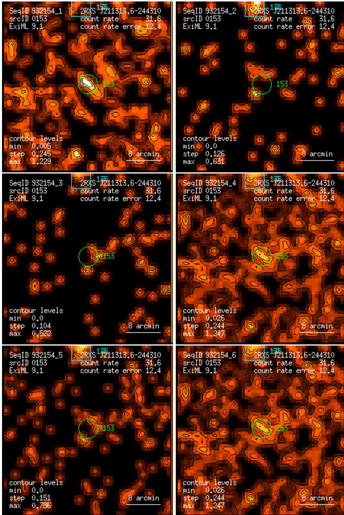
Figure 153: RASS 932154: detection 0153: band rate images, Gaussian filter: (1) PSPC channels 11 – 41, (2) 52 – 90, (3) 91 – 201, (4) 11 – 235, (5) 52 – 201, (6) 11 – 201. Broad band rates in counts/ks. Band rate contour levels in counts/ks/arcmin 2 .
