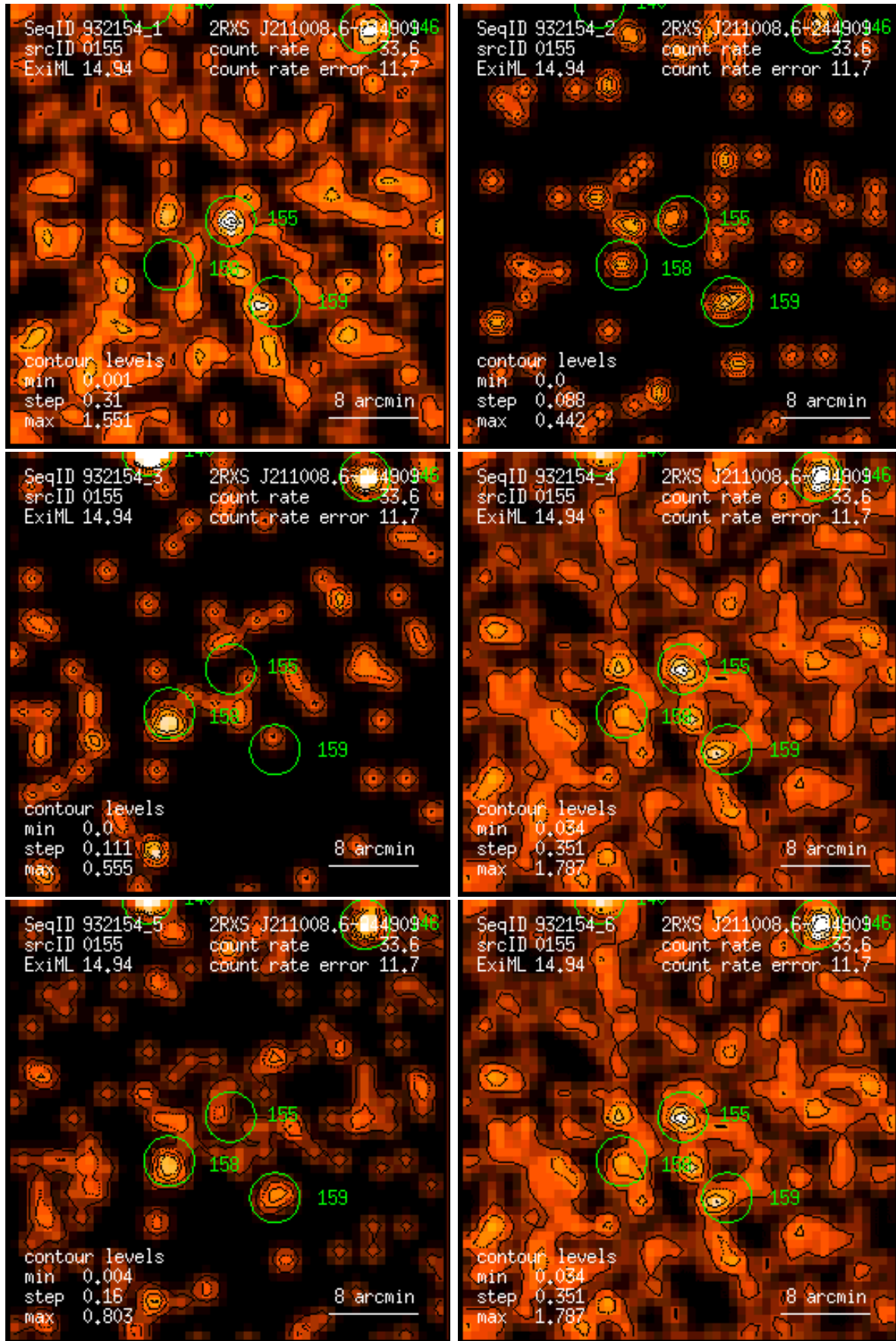
Figure 155: RASS 932154: detection 0155: band rate images, Gaussian filter: (1) PSPC channels 11 – 41, (2) 52 – 90, (3) 91 – 201, (4) 11 – 235, (5) 52 – 201, (6) 11 – 201. Broad band rates in counts/ks. Band rate contour levels in counts/ks/arcmin 2 .
