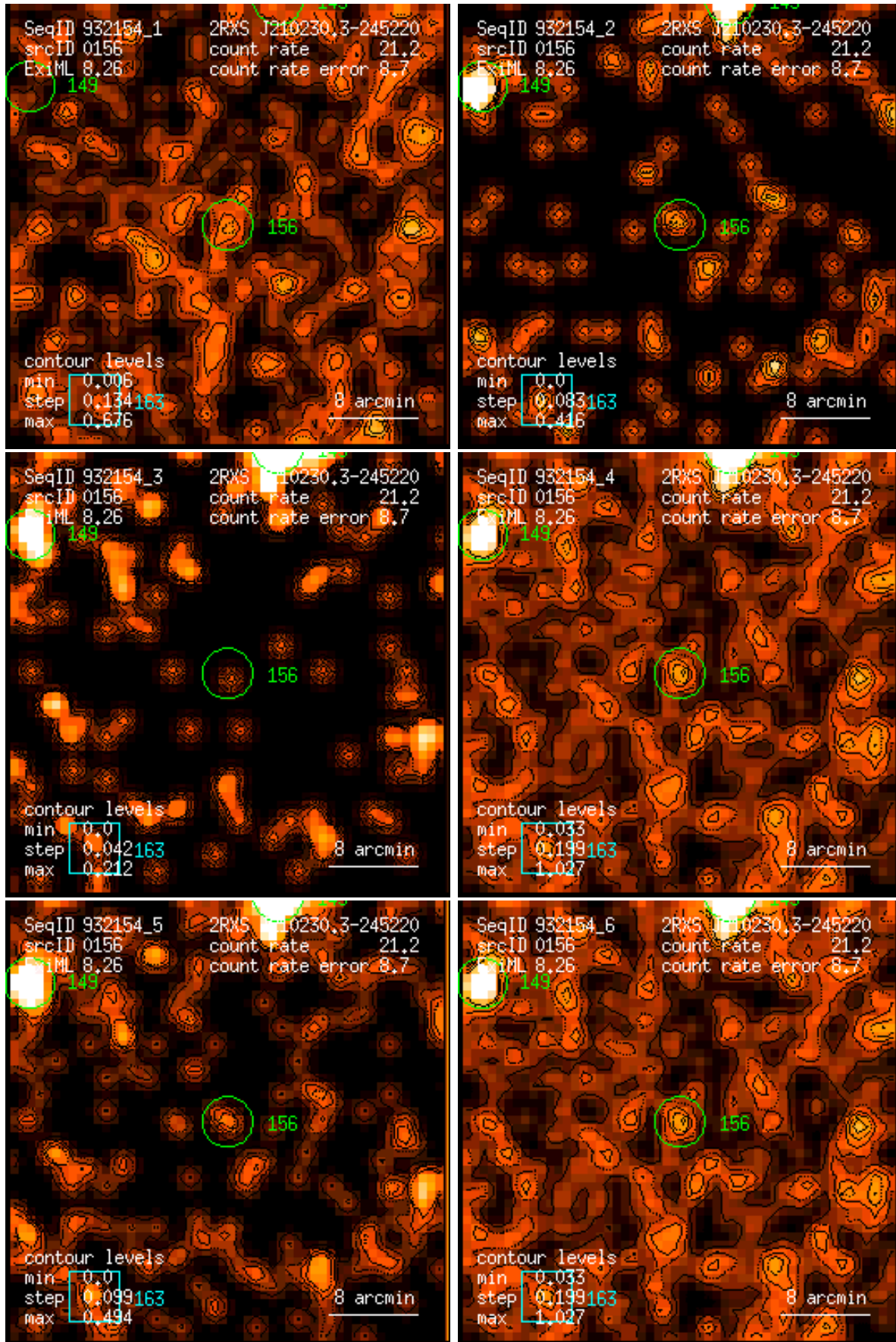
Figure 156: RASS 932154: detection 0156: band rate images, Gaussian filter: (1) PSPC channels 11 – 41, (2) 52 – 90, (3) 91 – 201, (4) 11 – 235, (5) 52 – 201, (6) 11 – 201. Broad band rates in counts/ks. Band rate contour levels in counts/ks/arcmin 2 .
