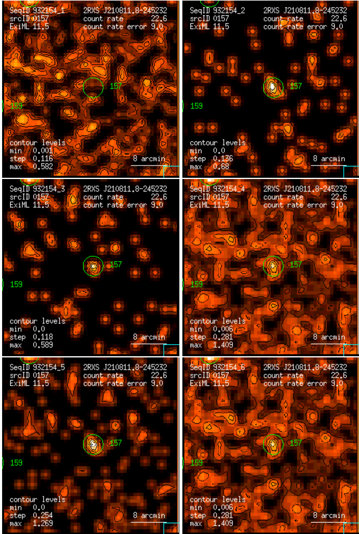
Figure 157: RASS 932154: detection 0157: band rate images, Gaussian filter: (1) PSPC channels 11 – 41, (2) 52 – 90, (3) 91 – 201, (4) 11 – 235, (5) 52 – 201, (6) 11 – 201. Broad band rates in counts/ks. Band rate contour levels in counts/ks/arcmin 2 .
