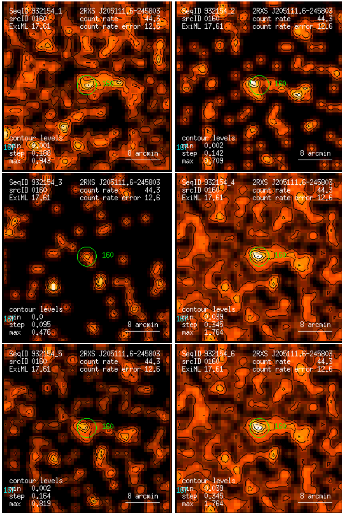
Figure 160: RASS 932154: detection 0160: band rate images, Gaussian filter: (1) PSPC channels 11 – 41, (2) 52 – 90, (3) 91 – 201, (4) 11 – 235, (5) 52 – 201, (6) 11 – 201. Broad band rates in counts/ks. Band rate contour levels in counts/ks/arcmin 2 .
