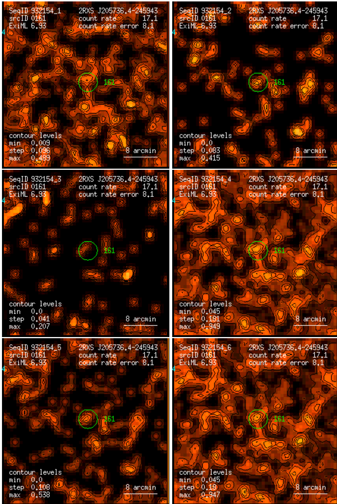
Figure 161: RASS 932154: detection 0161: band rate images, Gaussian filter: (1) PSPC channels 11 – 41, (2) 52 – 90, (3) 91 – 201, (4) 11 – 235, (5) 52 – 201, (6) 11 – 201. Broad band rates in counts/ks. Band rate contour levels in counts/ks/arcmin 2 .
