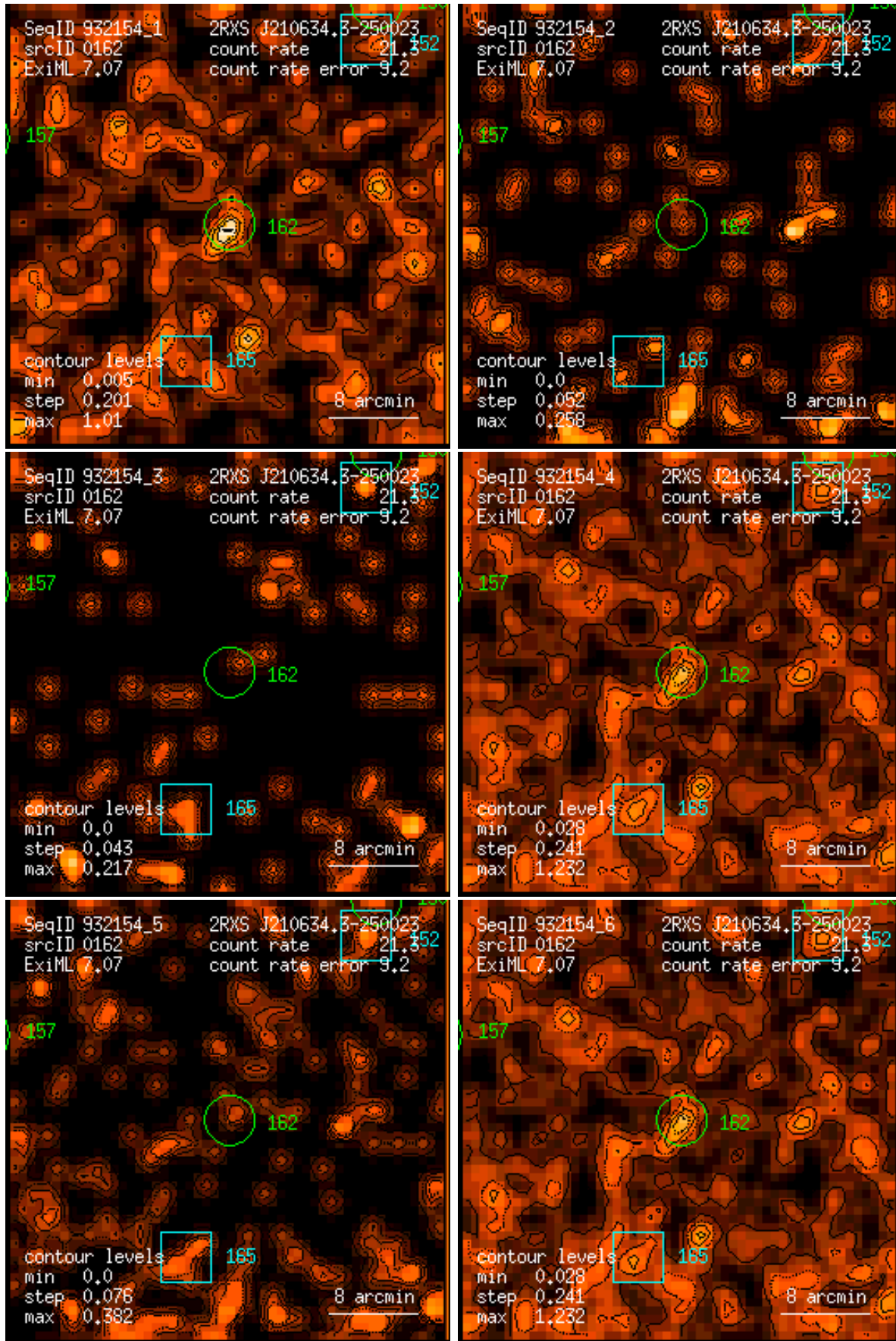
Figure 162: RASS 932154: detection 0162: band rate images, Gaussian filter: (1) PSPC channels 11 – 41, (2) 52 – 90, (3) 91 – 201, (4) 11 – 235, (5) 52 – 201, (6) 11 – 201. Broad band rates in counts/ks. Band rate contour levels in counts/ks/arcmin 2 .
