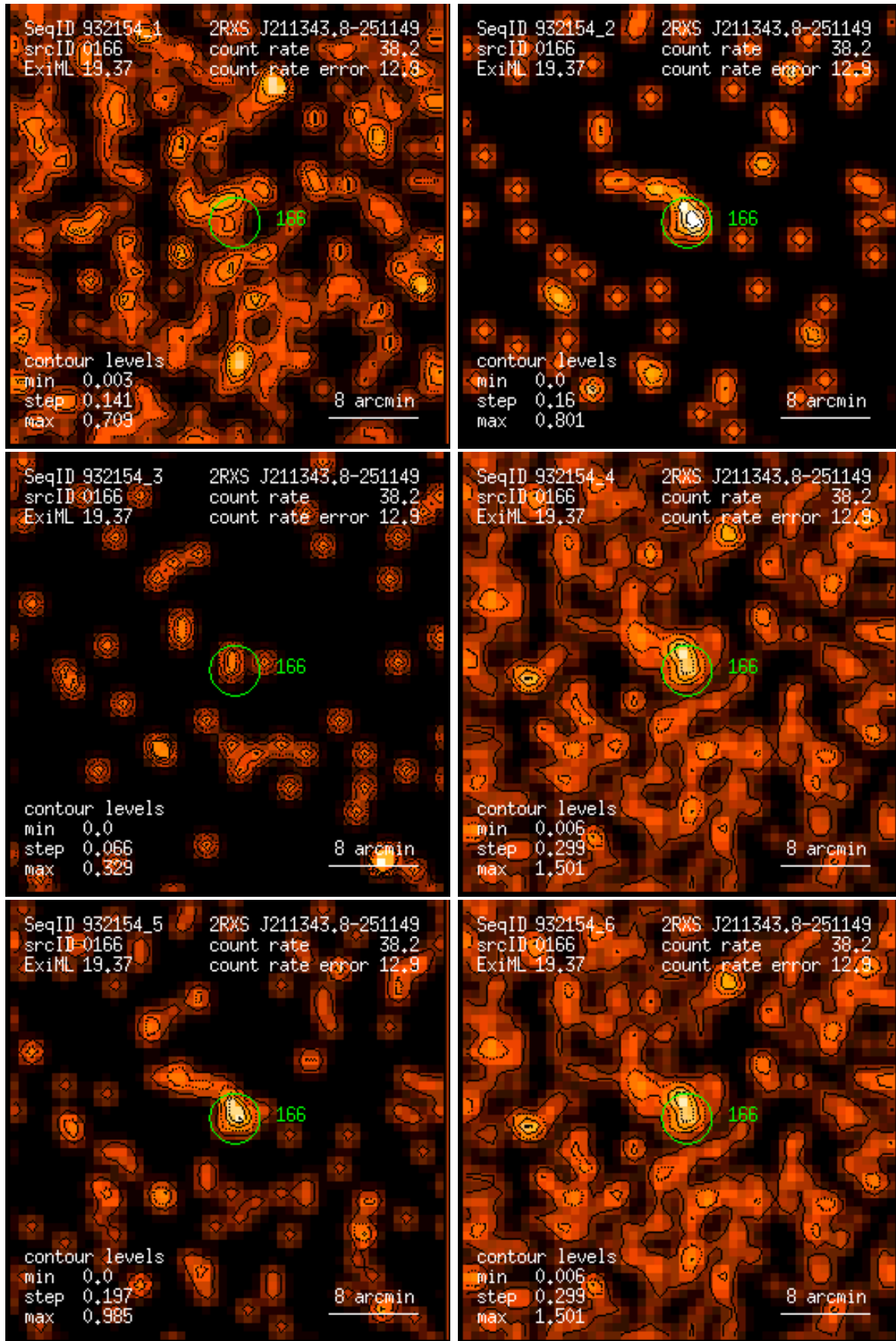
Figure 166: RASS 932154: detection 0166: band rate images, Gaussian filter: (1) PSPC channels 11 – 41, (2) 52 – 90, (3) 91 – 201, (4) 11 – 235, (5) 52 – 201, (6) 11 – 201. Broad band rates in counts/ks. Band rate contour levels in counts/ks/arcmin 2 .
