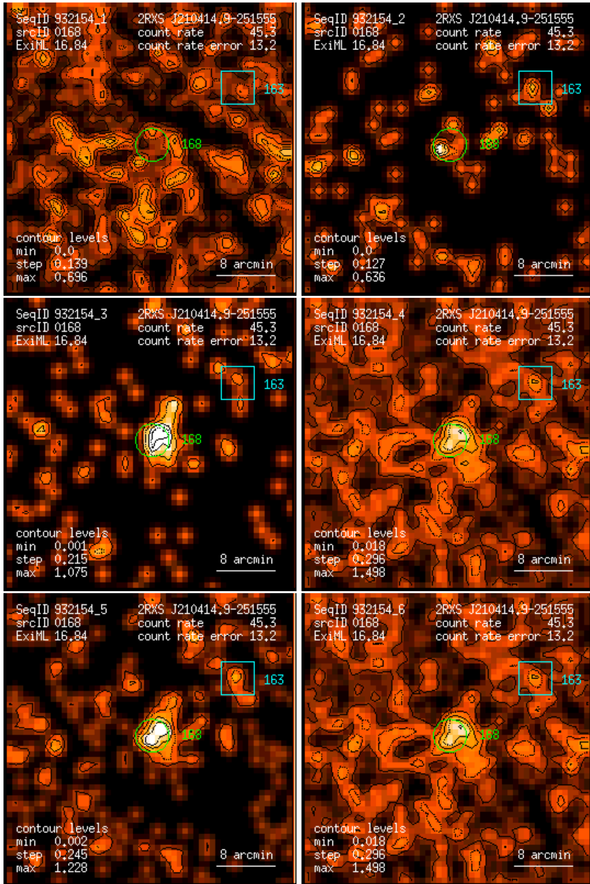
Figure 168: RASS 932154: detection 0168: band rate images, Gaussian filter: (1) PSPC channels 11 – 41, (2) 52 – 90, (3) 91 – 201, (4) 11 – 235, (5) 52 – 201, (6) 11 – 201. Broad band rates in counts/ks. Band rate contour levels in counts/ks/arcmin 2 .
