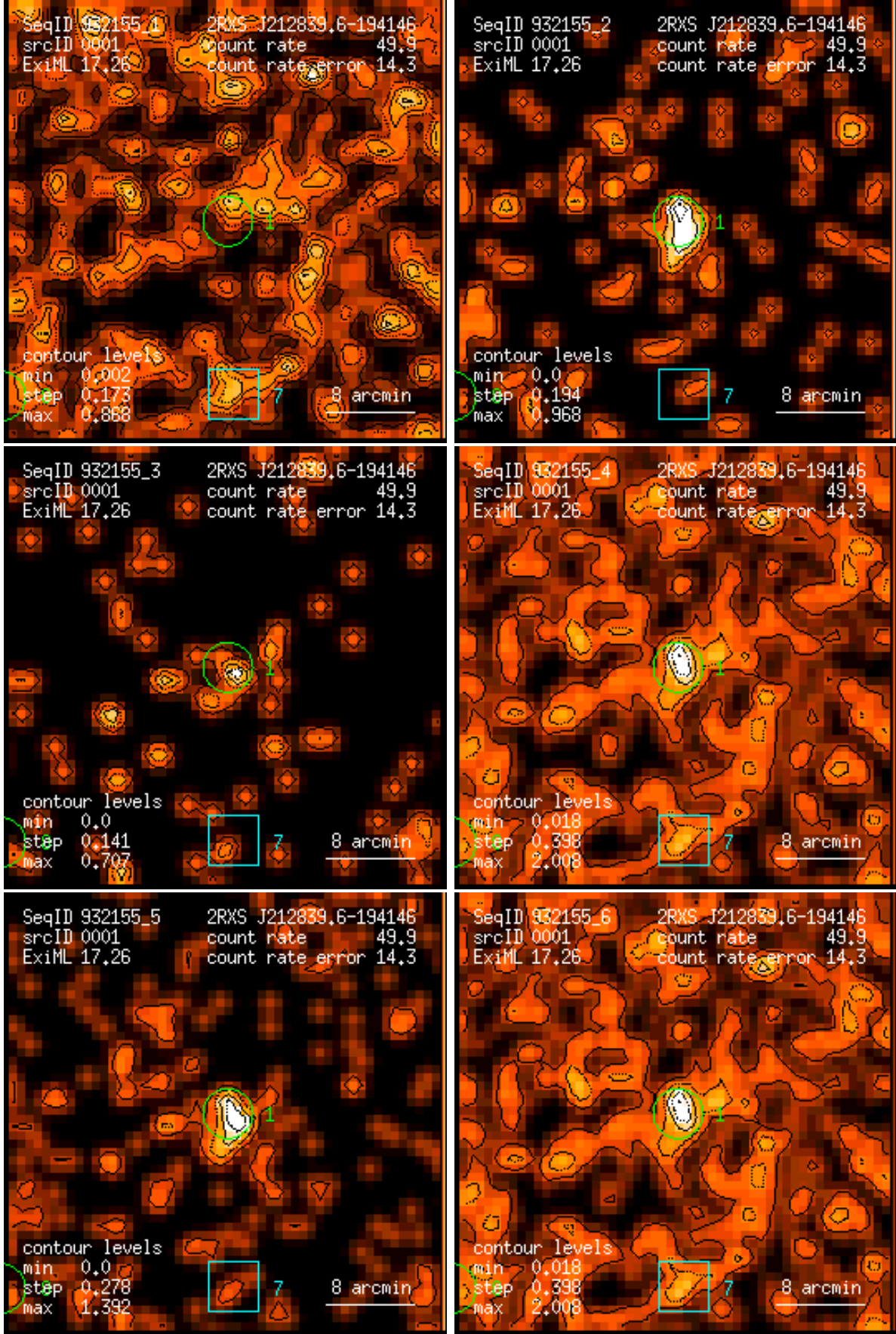
Figure 1: RASS 932155: detection 0001: band rate images, Gaussian filter: (1) PSPC channels 11 – 41, (2) 52 – 90, (3) 91 – 201, (4) 11 – 235, (5) 52 – 201, (6) 11 – 201. Broad band rates in counts/ks. Band rate contour levels in counts/ks/arcmin 2 .
