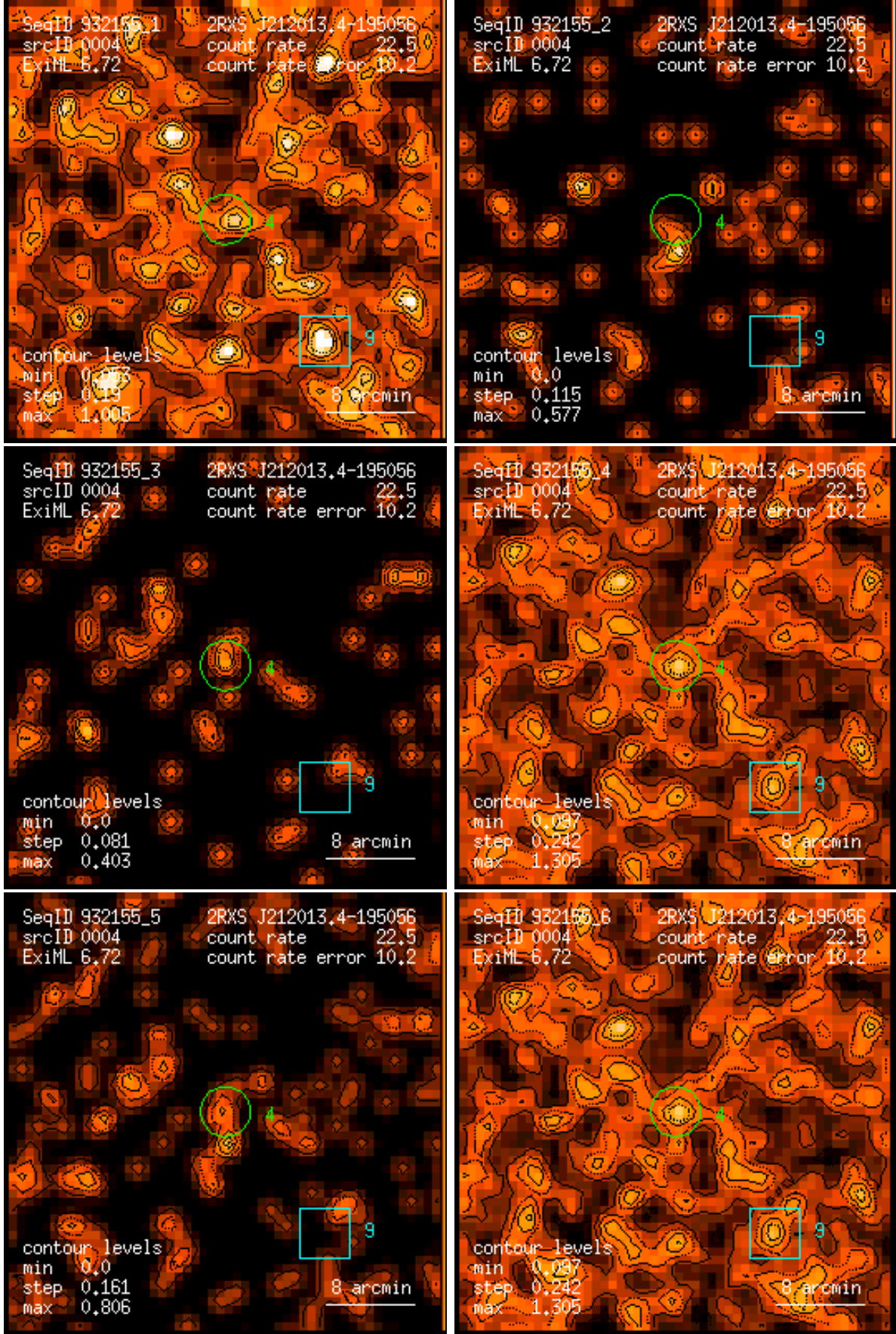
Figure 4: RASS 932155: detection 0004: band rate images, Gaussian filter: (1) PSPC channels 11 – 41, (2) 52 – 90, (3) 91 – 201, (4) 11 – 235, (5) 52 – 201, (6) 11 – 201. Broad band rates in counts/ks. Band rate contour levels in counts/ks/arcmin 2 .
