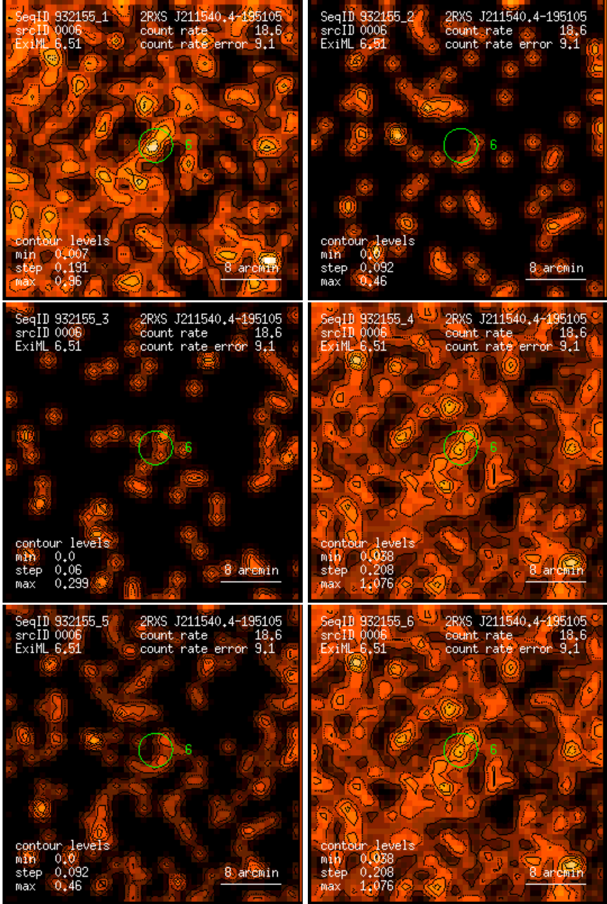
Figure 6: RASS 932155: detection 0006: band rate images, Gaussian filter: (1) PSPC channels 11 – 41, (2) 52 – 90, (3) 91 – 201, (4) 11 – 235, (5) 52 – 201, (6) 11 – 201. Broad band rates in counts/ks. Band rate contour levels in counts/ks/arcmin 2 .
