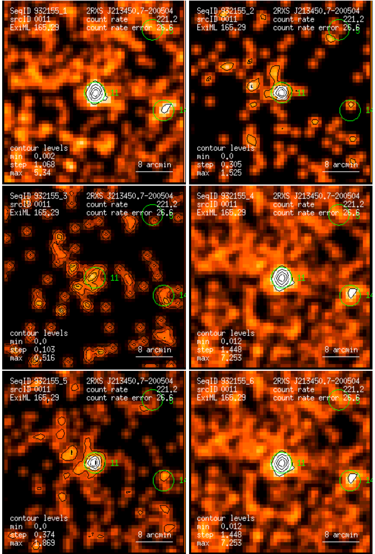
Figure 11: RASS 932155: detection 0011: band rate images, Gaussian filter: (1) PSPC channels 11 – 41, (2) 52 – 90, (3) 91 – 201, (4) 11 – 235, (5) 52 – 201, (6) 11 – 201. Broad band rates in counts/ks. Band rate contour levels in counts/ks/arcmin 2 .
