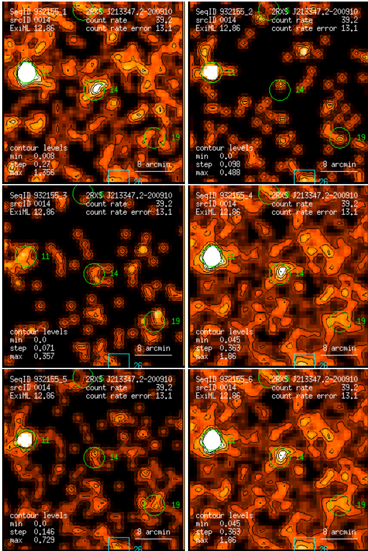
Figure 14: RASS 932155: detection 0014: band rate images, Gaussian filter: (1) PSPC channels 11 – 41, (2) 52 – 90, (3) 91 – 201, (4) 11 – 235, (5) 52 – 201, (6) 11 – 201. Broad band rates in counts/ks. Band rate contour levels in counts/ks/arcmin 2 .
