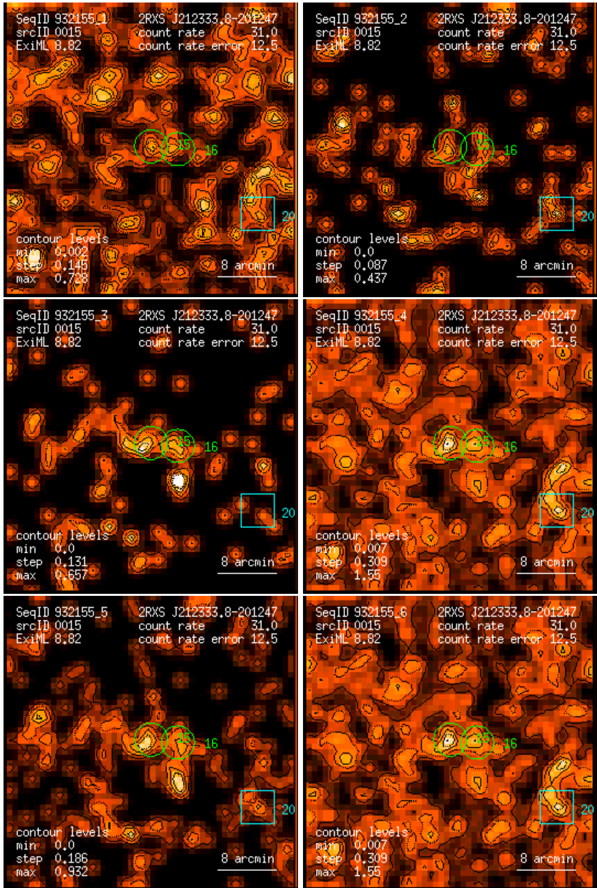
Figure 15: RASS 932155: detection 0015: band rate images, Gaussian filter: (1) PSPC channels 11 – 41, (2) 52 – 90, (3) 91 – 201, (4) 11 – 235, (5) 52 – 201, (6) 11 – 201. Broad band rates in counts/ks. Band rate contour levels in counts/ks/arcmin 2 .
