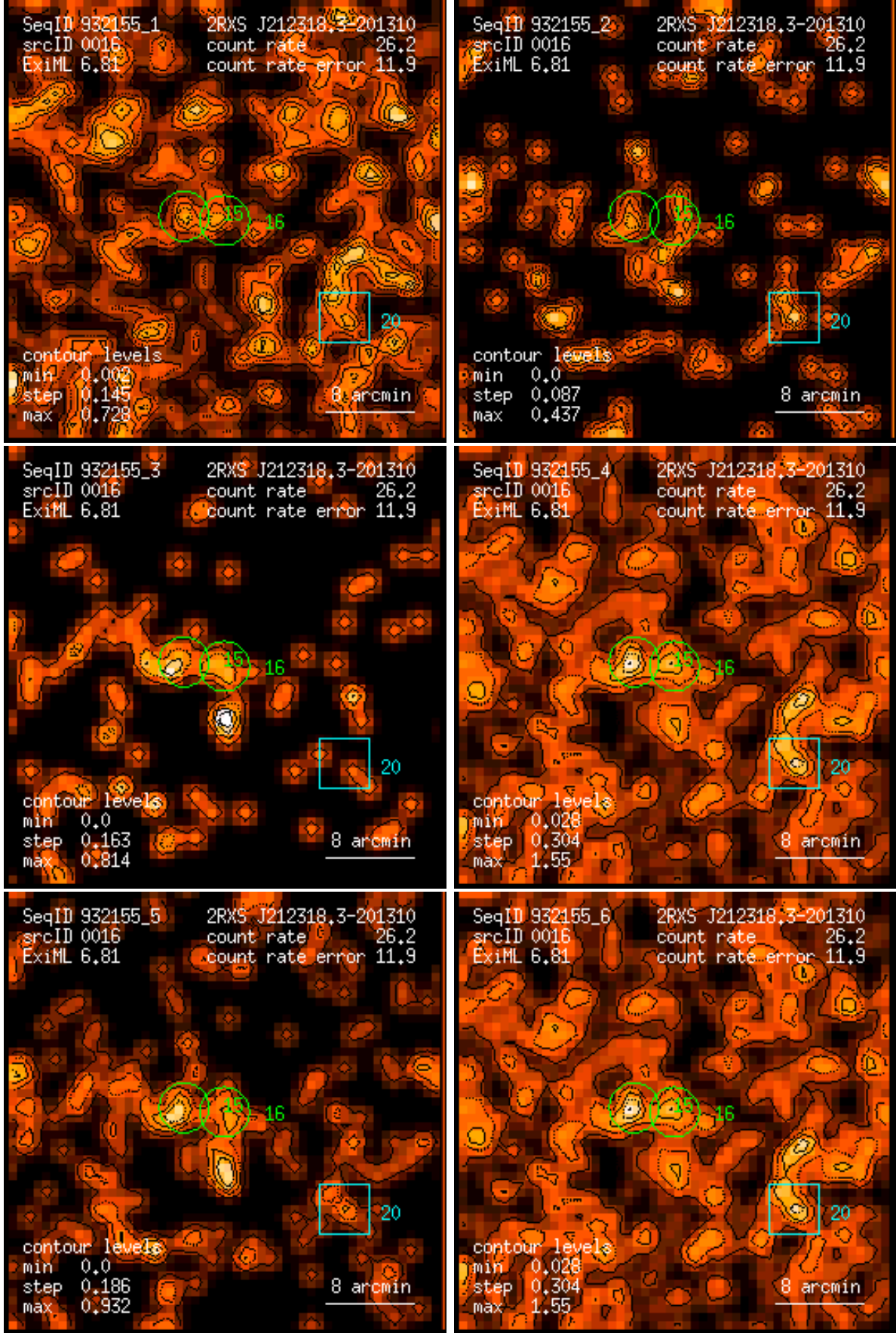
Figure 16: RASS 932155: detection 0016: band rate images, Gaussian filter: (1) PSPC channels 11 – 41, (2) 52 – 90, (3) 91 – 201, (4) 11 – 235, (5) 52 – 201, (6) 11 – 201. Broad band rates in counts/ks. Band rate contour levels in counts/ks/arcmin 2 .
