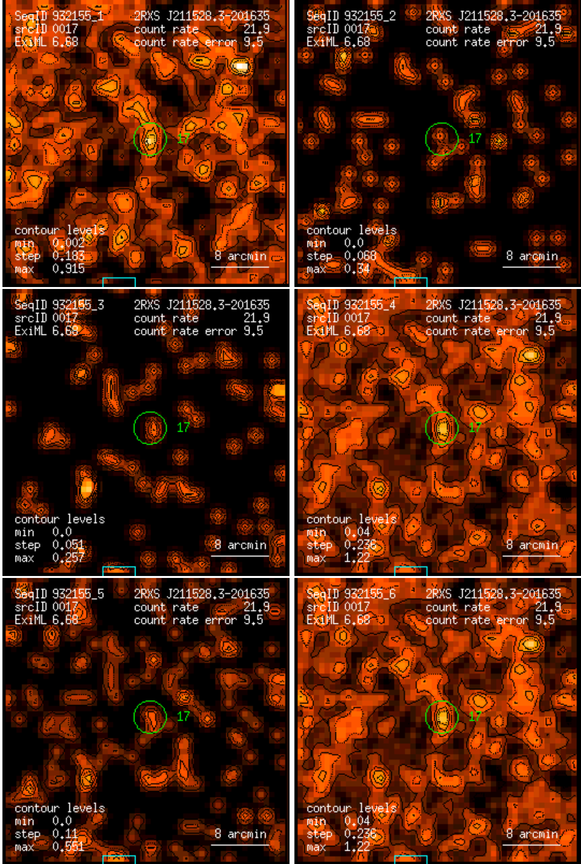
Figure 17: RASS 932155: detection 0017: band rate images, Gaussian filter: (1) PSPC channels 11 – 41, (2) 52 – 90, (3) 91 – 201, (4) 11 – 235, (5) 52 – 201, (6) 11 – 201. Broad band rates in counts/ks. Band rate contour levels in counts/ks/arcmin 2 .
