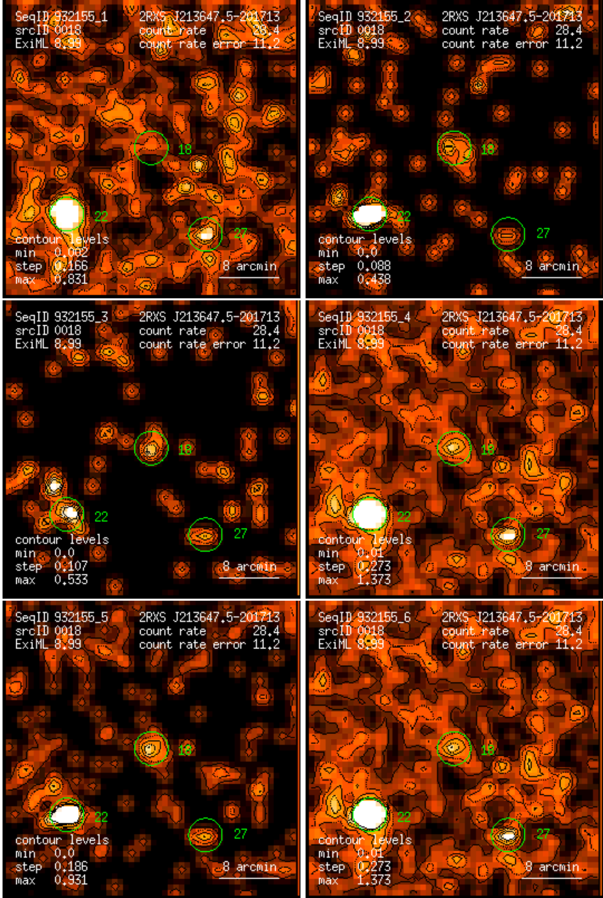
Figure 18: RASS 932155: detection 0018: band rate images, Gaussian filter: (1) PSPC channels 11 – 41, (2) 52 – 90, (3) 91 – 201, (4) 11 – 235, (5) 52 – 201, (6) 11 – 201. Broad band rates in counts/ks. Band rate contour levels in counts/ks/arcmin 2 .
