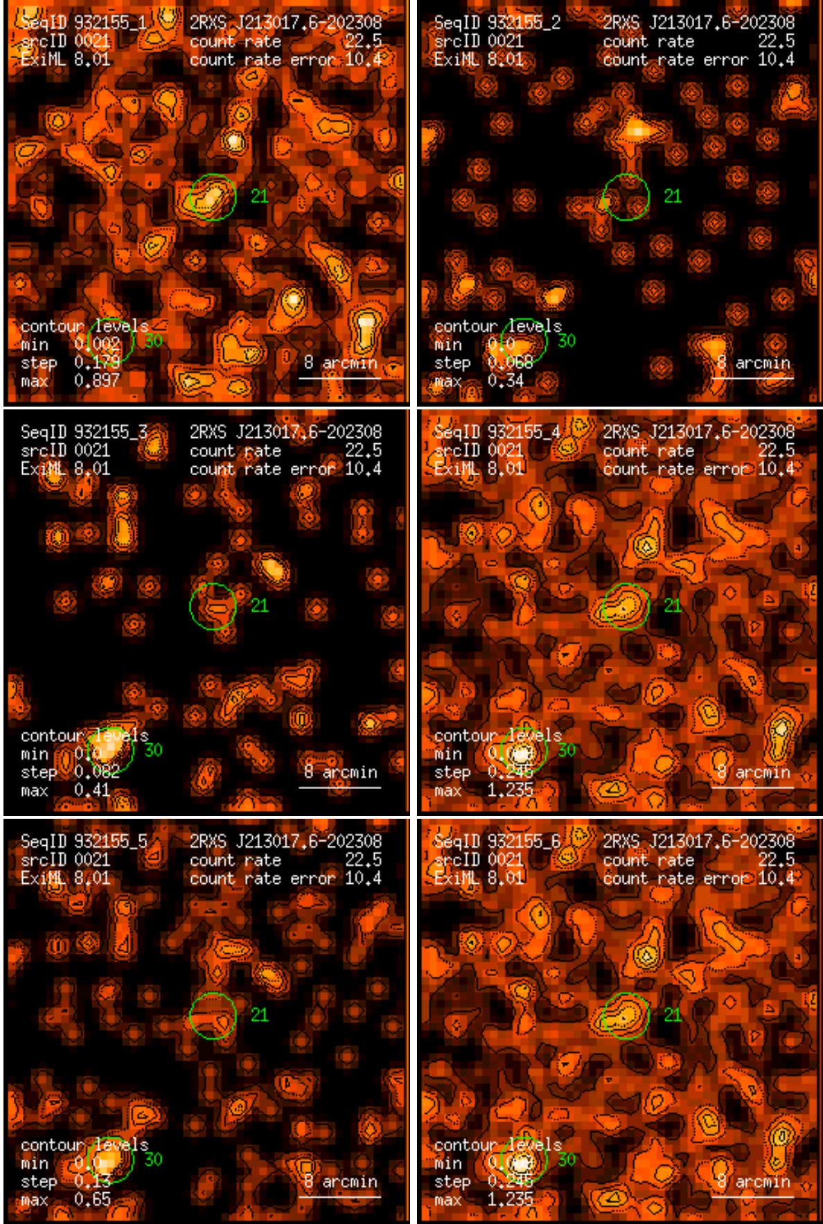
Figure 21: RASS 932155: detection 0021: band rate images, Gaussian filter: (1) PSPC channels 11 – 41, (2) 52 – 90, (3) 91 – 201, (4) 11 – 235, (5) 52 – 201, (6) 11 – 201. Broad band rates in counts/ks. Band rate contour levels in counts/ks/arcmin 2 .
