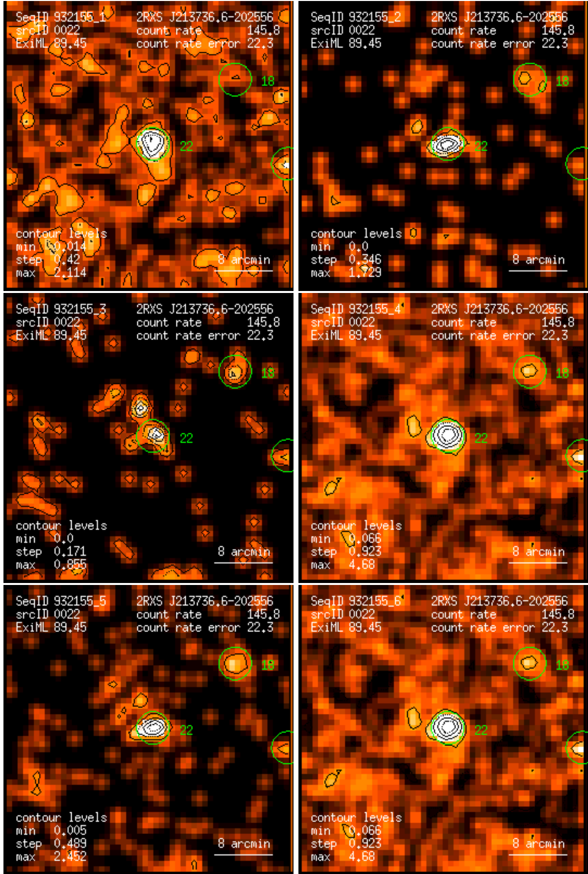
Figure 22: RASS 932155: detection 0022: band rate images, Gaussian filter: (1) PSPC channels 11 – 41, (2) 52 – 90, (3) 91 – 201, (4) 11 – 235, (5) 52 – 201, (6) 11 – 201. Broad band rates in counts/ks. Band rate contour levels in counts/ks/arcmin 2 .
