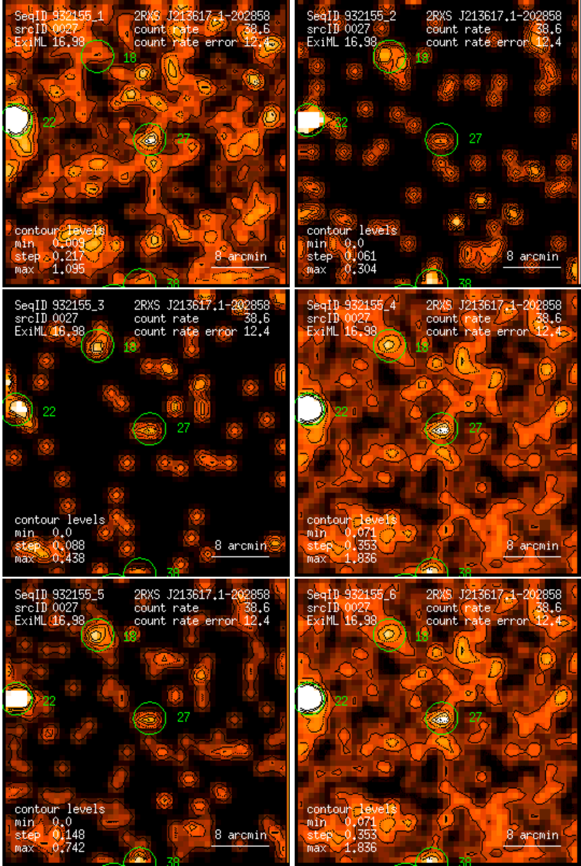
Figure 27: RASS 932155: detection 0027: band rate images, Gaussian filter: (1) PSPC channels 11 – 41, (2) 52 – 90, (3) 91 – 201, (4) 11 – 235, (5) 52 – 201, (6) 11 – 201. Broad band rates in counts/ks. Band rate contour levels in counts/ks/arcmin 2 .
