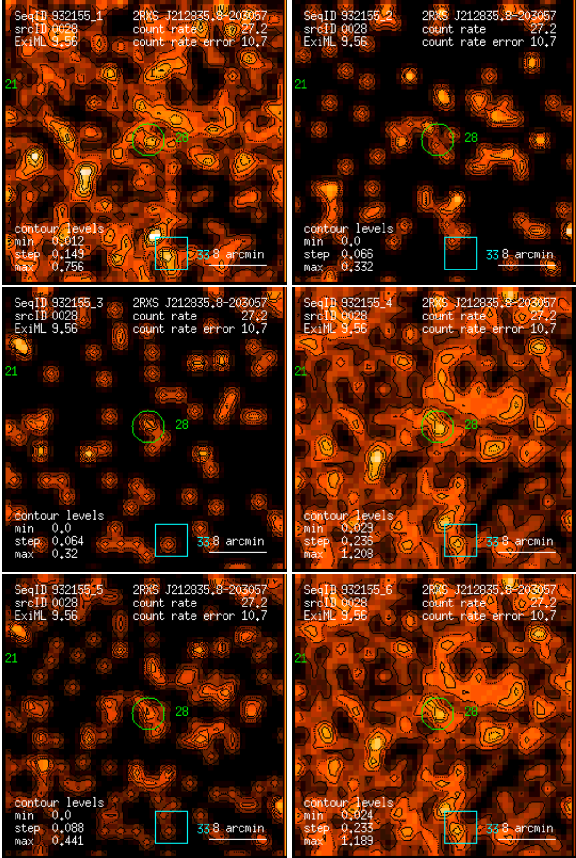
Figure 28: RASS 932155: detection 0028: band rate images, Gaussian filter: (1) PSPC channels 11 – 41, (2) 52 – 90, (3) 91 – 201, (4) 11 – 235, (5) 52 – 201, (6) 11 – 201. Broad band rates in counts/ks. Band rate contour levels in counts/ks/arcmin 2 .
